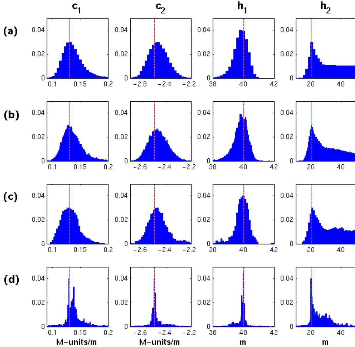
Figure 4 Marginal posterior probability distributions for the synthetic test case. Vertical lines show the true values of the parameters. (a) exhaustive search, (b) Metropolis algorithm, (c) Gibbs algorithm, and (d) genetic algorithm.
