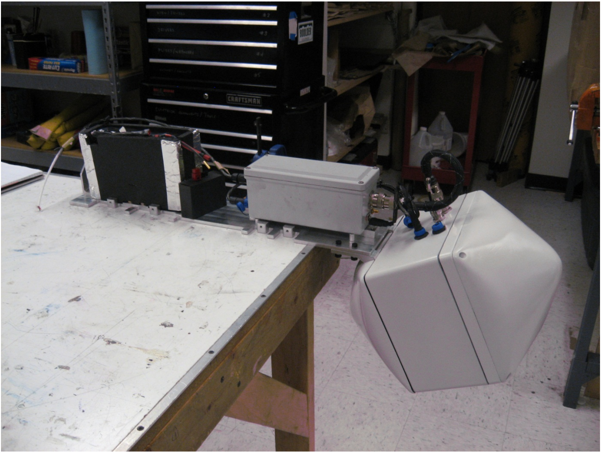
Figure 3a: CULPIS-X in CU-Boulder Lab. Sensor package on right, data acquisition box in middle, battery on left
