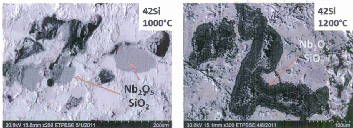
Figure 27 Oxidation features at the microscopic level for 42Si alloy.
