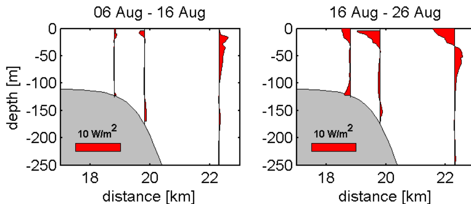
Figure 5: Energy flux profiles near the shelfbreak during periods of weak (left) and strong (right) NLIW activity. A 5 \text{ W/m}^2 onshore internal tide occurs at all stations during strong NLIW activity.
