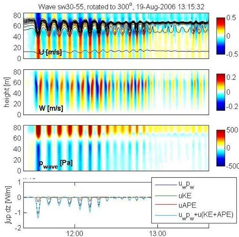
Figure 2: Example computation of the nonlinear, nonhydrostatic internal wave energy and energy flux.
