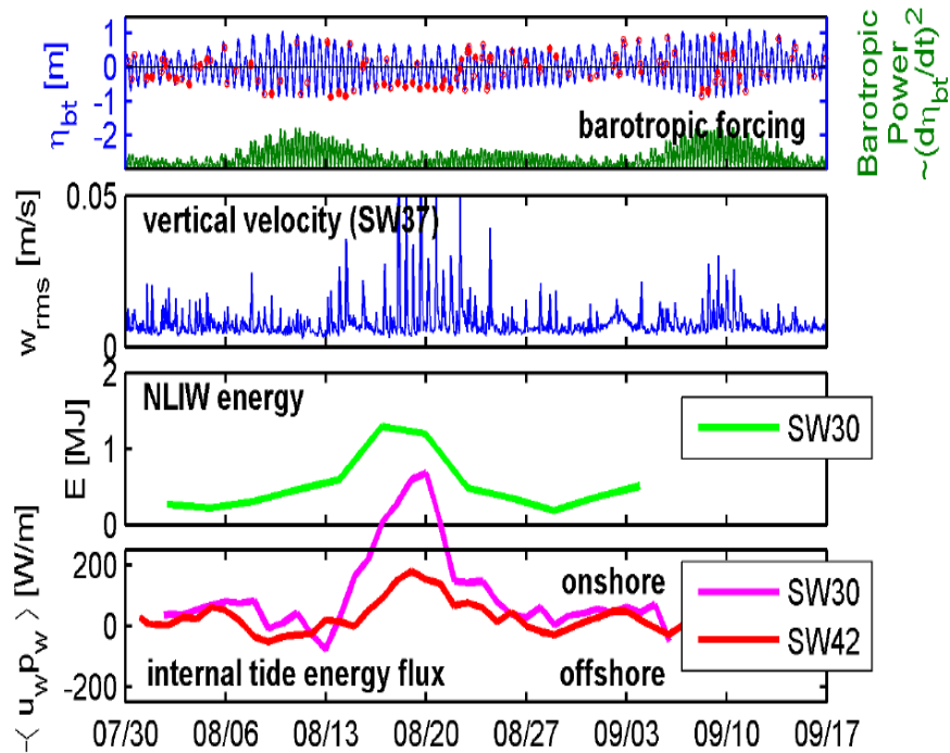
Figure 3: Summary of NLIW temporal variability. Forcing by the barotropic tide (elevation & power; top row) is poorly correlated with NLIW vertical velocity at SW37, the 70-m isobath (2 nd row). Red dots in upper panel represent wave arrival times at SW37. The resultant NLIW energy (3 rd row) is found to covary with the internal tide energy flux (bottom row).
