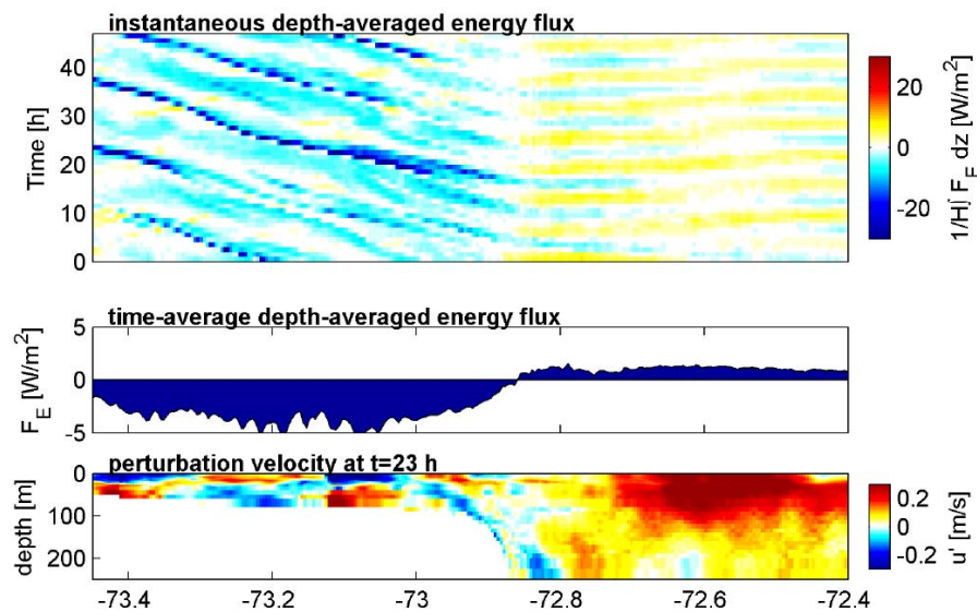
Figure 6: Analysis of Gallacher's numerical simulations for a 48 h period during July 2006. Top shows instantaneous depth-averaged energy flux, which radiates from the shelf break in sporadic events. Middle shows depth averaged energy flux. A snapshot of perturbation velocity (bottom) shows that the internal tide produces a bore-like pulse of fluid at -73.1 W where it reflects with the surface. This may provides hints to the NLIW generation process.
