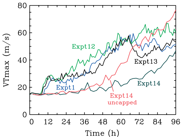
Figure A.3. Time series of VT_{\max} through to 4 days for Experiments 12–14 (see text for details). Also shown for reference is the time series of VT_{\max} for Experiment 1 and the uncapped counterpart of Experiment 14.
