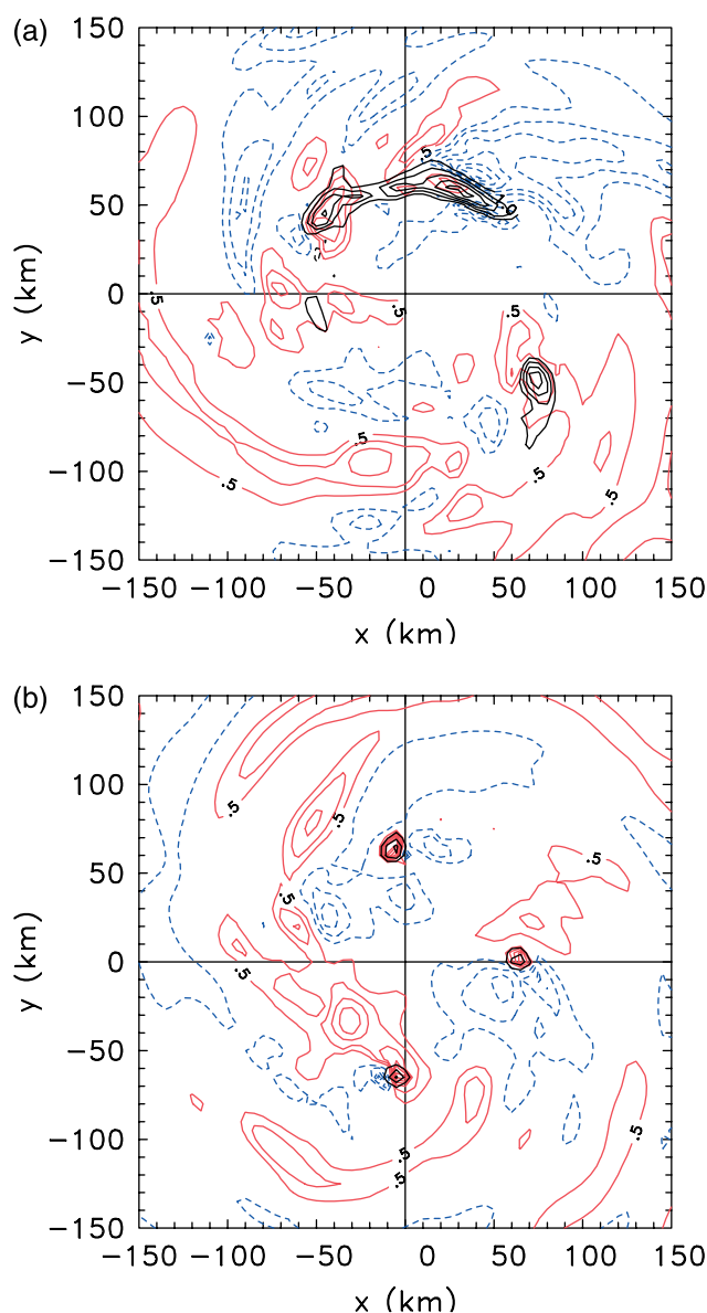
Figure 6. Horizontal cross-section at 5 \text{ km} altitude of the deviation of density temperature from the azimuthal mean field for (a) Experiment 1 at 60 hours and (b) the corresponding virtual temperature deviation for Experiment 2 at 24 hours. Positive values of temperature deviation are denoted by solid contours and negative values by dashed contours; the contour interval is 0.5 \text{ K} . The vertical velocity at the same level (black contours) is superimposed to corroborate the juxtaposition of regions of strong upward motion and local warmth. The contour interval is 1 \text{ m s}^{-1} for (a) (warm rain) and 5 \text{ m s}^{-1} for (b) (pseudo-adiabatic).
