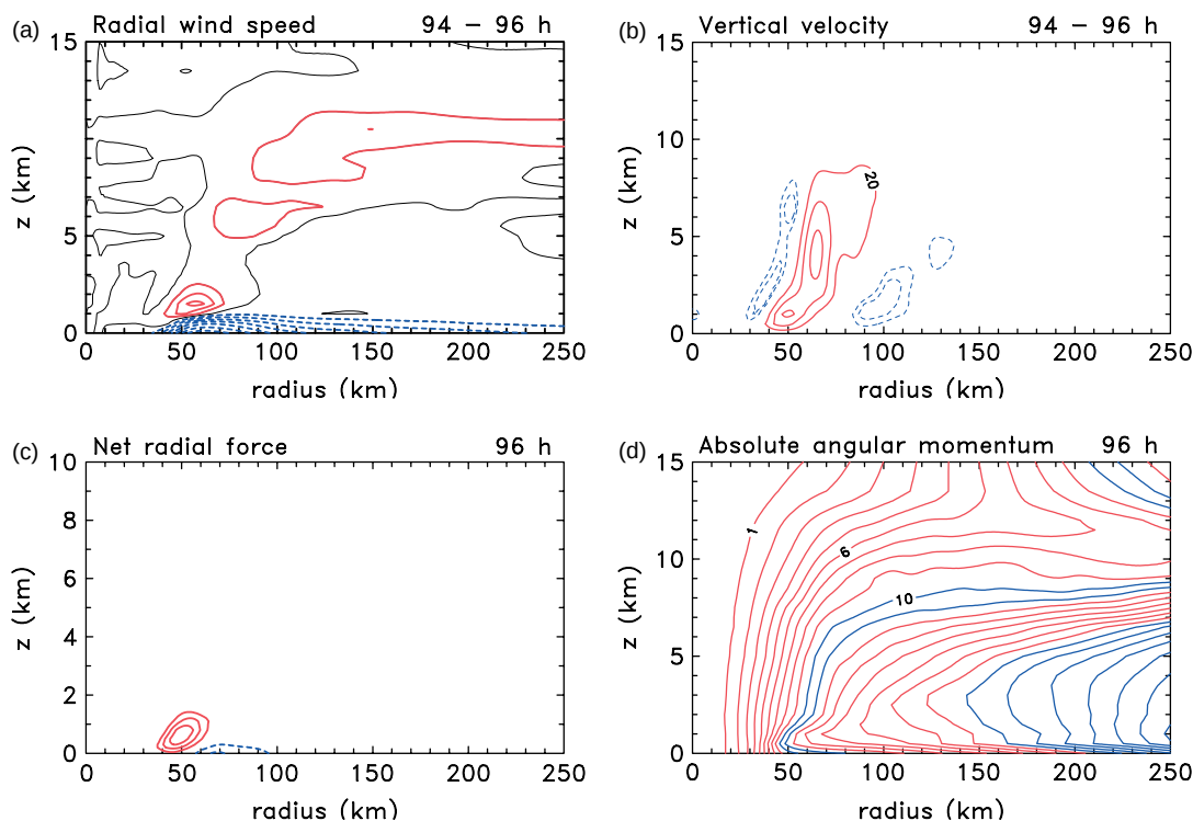
Figure 9. Radius–height cross-sections of isopleths in the warm-rain calculation at 96 hours: (a) radial velocity (contour interval 2\text{ m s}^{-1} ; positive bold solid and negative dashed, with thin zero line); (b) vertical velocity (contour interval 20\text{ cm s}^{-1} for positive (solid) values and 2\text{ cm s}^{-1} for negative (dashed) values); (c) net radial force (contour interval 1.5\text{ m s}^{-1}\text{ h}^{-1} , with solid curves indicating positive values, dashed curves negative values; zero contours are not shown); (d) absolute angular momentum (contour interval 1 \times 10^6\text{ m}^2\text{ s}^{-1} ). These figures should be compared with Figures 5(c,d), 6(c) and 7(d), respectively. This figure is available in colour online at www.interscience.wiley.com/journal/qj
