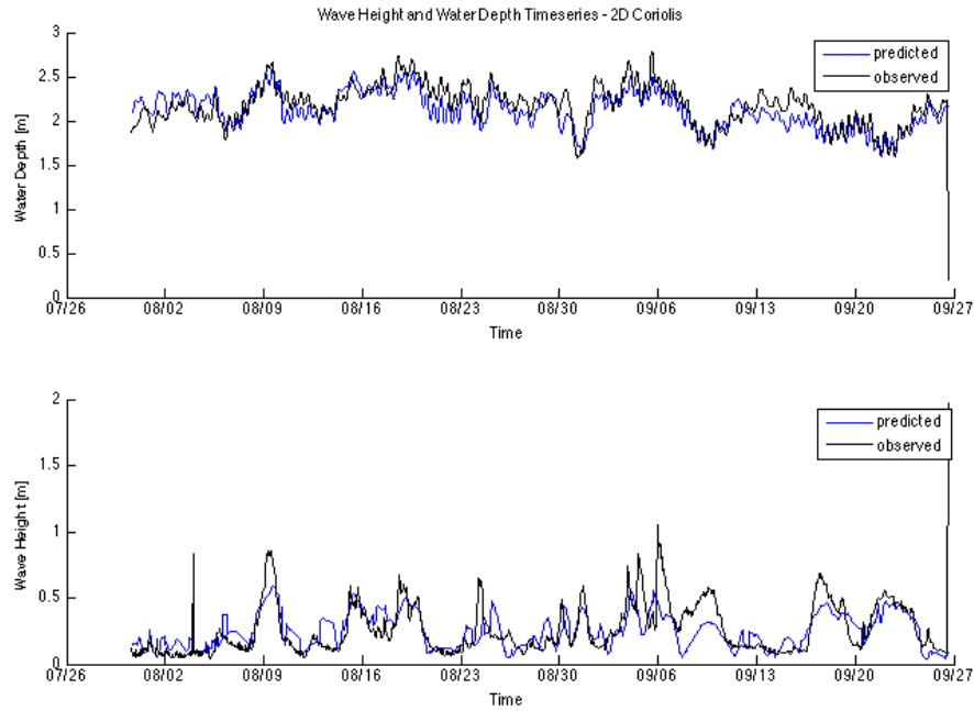
Figure 12 Observed and predicted timeseries of water depth and wave height from summer 2009. Modeled timeseries will be constructed for the timeperiod 1979-2012 and used as drivers for hindcast model runs.
