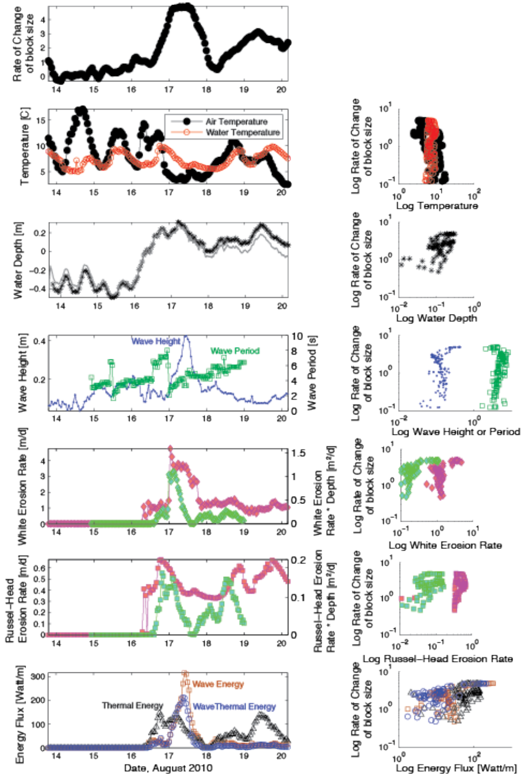
Figure 10. Comparison of the rate of change of apparent area of the block shown in Figure 9 with all observed environmental conditions (air temperature, water temperature, water level, wave height, wave period), and theoretical rules for instantaneous submarine erosion rate (White, Russell-Head, Wave Energy, Thermal Energy).
