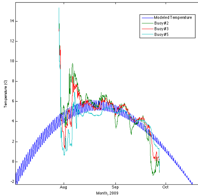
Figure 12. Modeled and measured (at 3 locations) water temperature from summer 2009. Water temperature model captures the seasonal and daily cycles of water temperature but does not capture variations in water temperature associated with passing storms (few day-week time scale).
