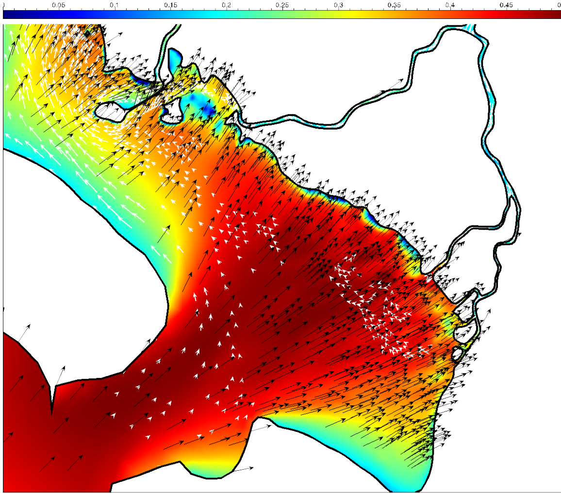
Fig. 9: Model-computed significant wave height (m) at high tide under steady state 15 knot SW wind forcing. Wave direction (black arrows) and Vertically-averaged velocity (white arrows).
