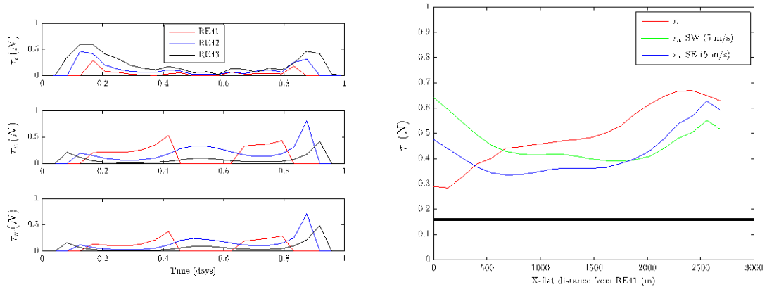
Fig. 6: [Left] Bed stress over a spring tidal cycle at three cross flat locations. Upper panel: stress due to currents. Middle panel: wave-induced stress driven by SW winds at 5 m/s. Lower panel: wave-induced stress driven by SE winds at 5 m/s. [Right] Cross-flat profile of maximum bed stress over a spring-neap cycle. Critical shear stress of dominant grain size on the Skagit flats ( \phi=2.5 ) shown for reference (black line).
