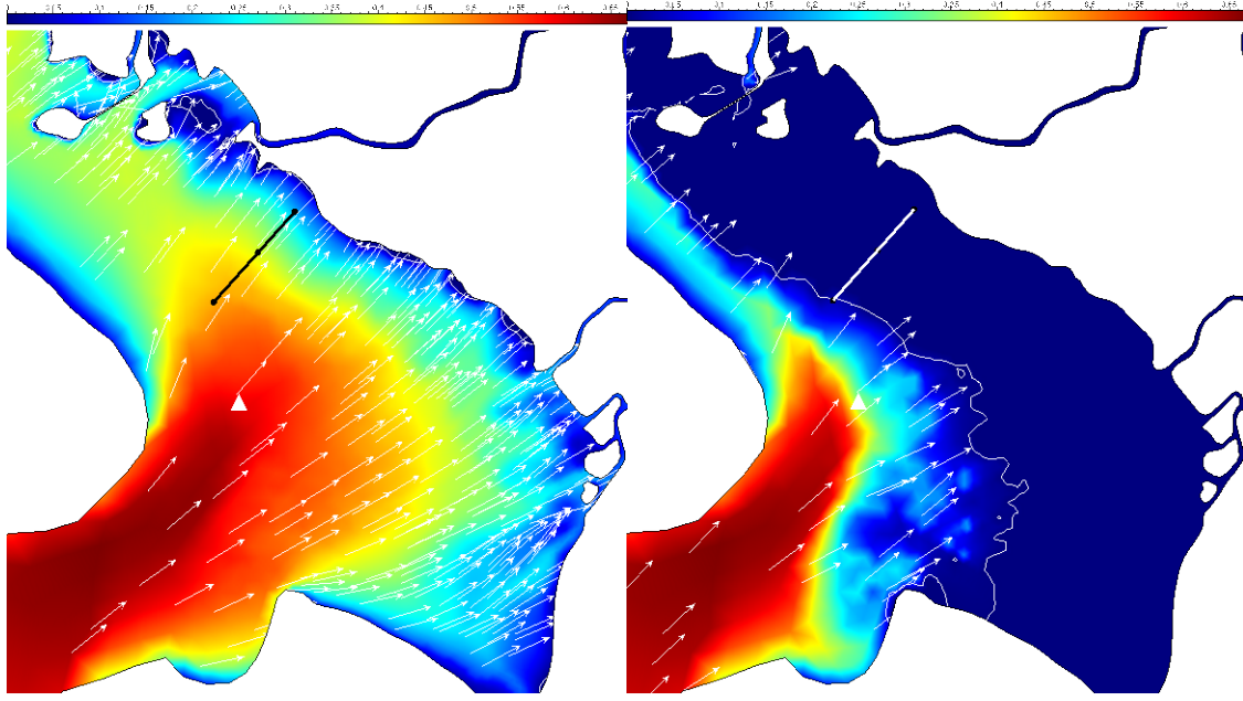
Fig. 2: Wave direction vectors and significant wave height for a SW wind at 10 m/s during spring high tide (left) and spring low tide (right)
