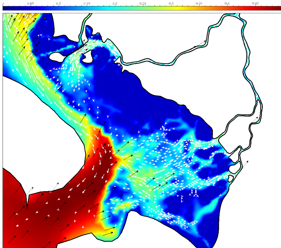
Fig. 8: Model-computed significant wave height (m) at low tide under steady state 15 knot SW wind forcing. Wave direction (black arrows) and Vertically-averaged velocity (white arrows).
