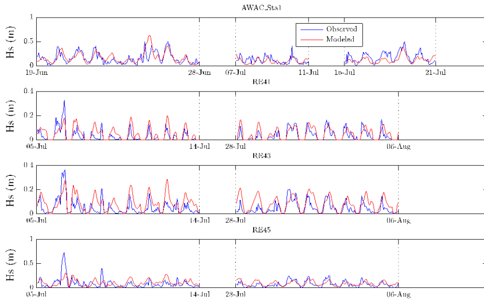
Fig. 3: Comparison of model-computed and observed significant wave height during several wind events in summer, 2009. For station locations, see Figure 1.
