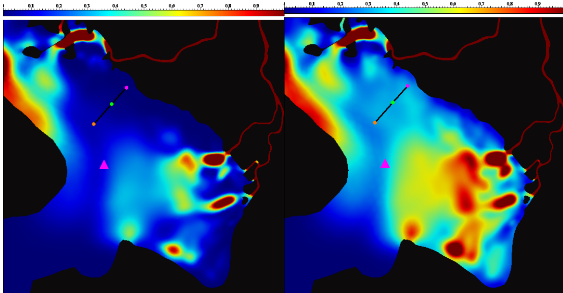
Fig. 7: Model-computed cumulative erosion in meters for the Skagit Flats for the period June 1, 2009 through Sep 1, 2009. Left panel: Currents only. Right panel: Currents and Waves
