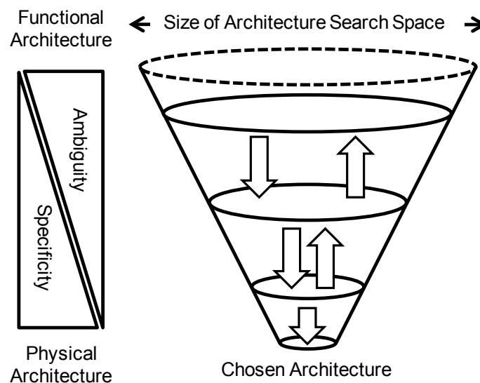
Figure 3.1. Ambiguity Reductions in the Architecture Search Process
