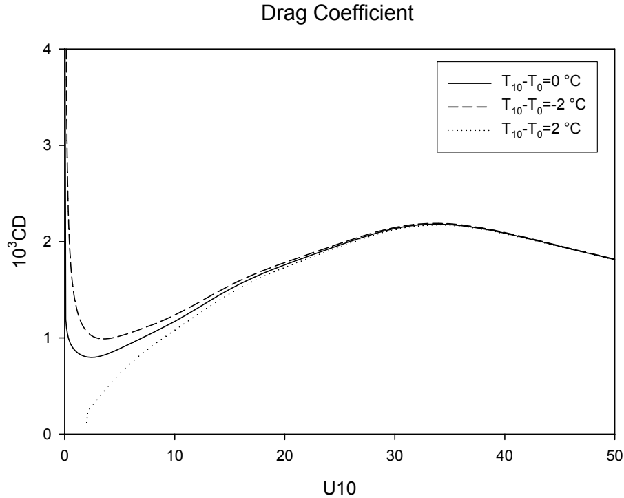
Figure 2. Drag coefficient that results from the wind profiles shown as a function of wind speed and for stable (dot) unstable (dash) and neutral (solid) conditions.
