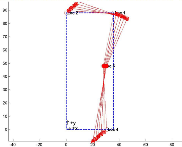
APG B2006, 5 Nov 2004, hammer impacts @ C; ODS for mean resonant frequency = 11.7886 Hz
