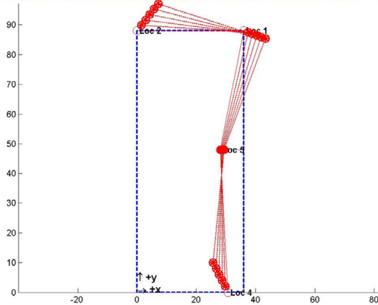
APG B2006, 5 Nov 2004, hammer impacts @ C; ODS for mean resonant frequency = 11.0857 Hz
