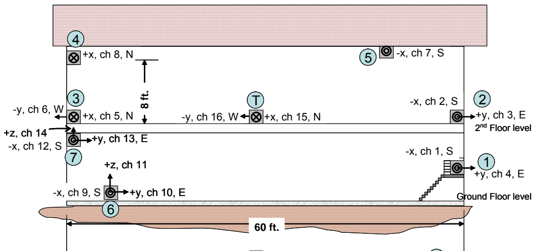
Figure 3-10. Plan Schematic Showing Numbered Locations and Orientations of Accelerometers for the Ceiling Level Above the Second Floor
