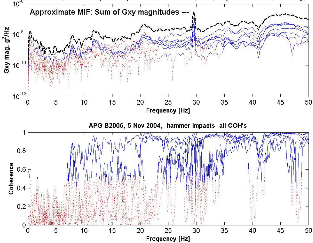
Figure 4-30. Example of Overlaid Functions for CSD Phase, CSD Magnitude and Coherence for Entire Set of Response Measurements
