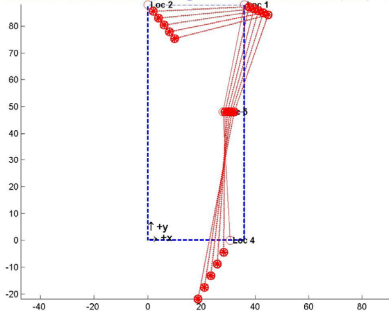
APG B2006, 5 Nov 2004, hammer impacts @ C; ODS for mean resonant frequency = 13.5086 Hz
