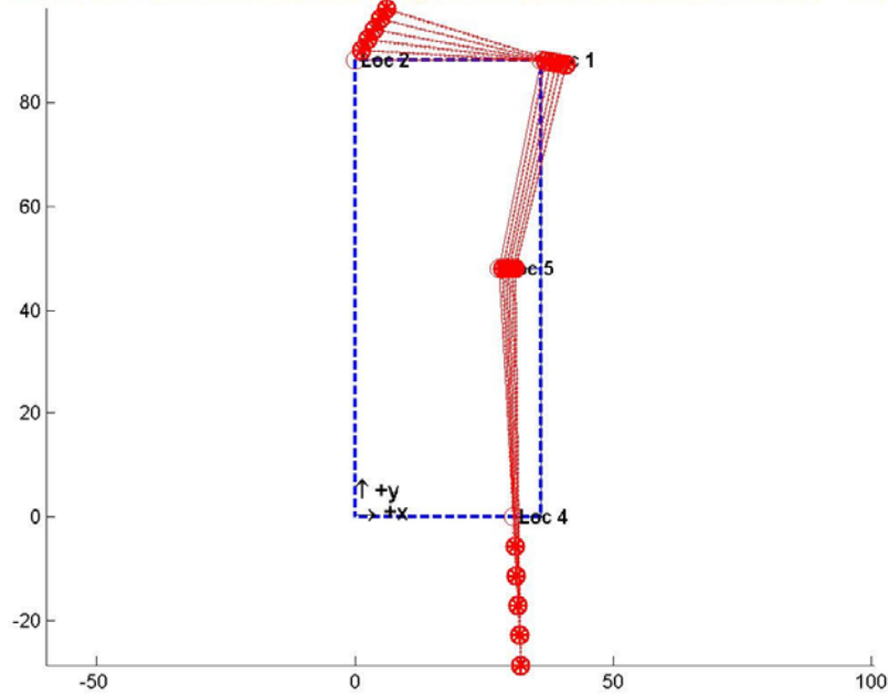
APG B2006, 5 Nov 2004, hammer impacts @ C; ODS for mean resonant frequency = 19.3029 Hz
