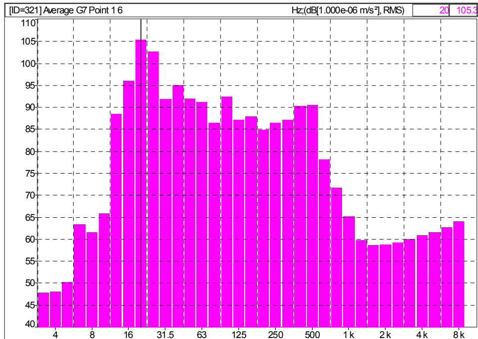
(b) Glass acceleration power spectrum, dB re 1 μm/sec², versus band center frequency, Hz
