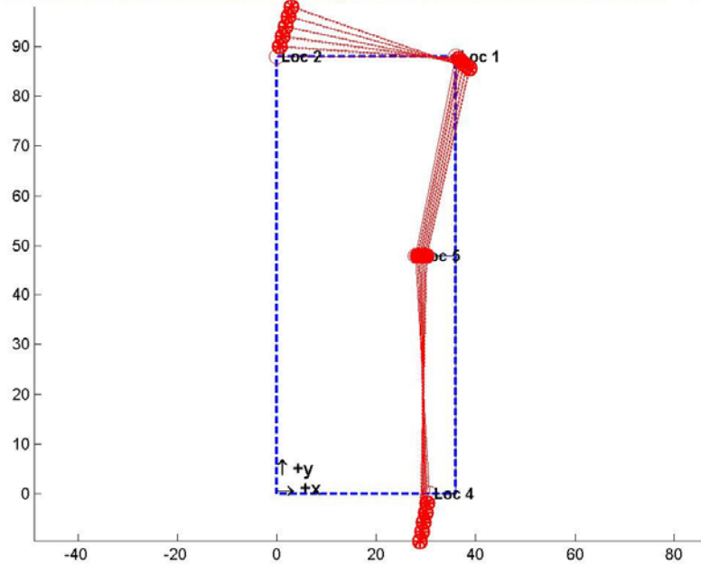
APG B2006, 5 Nov 2004, hammer impacts @ C; ODS for mean resonant frequency = 10.2629 Hz
