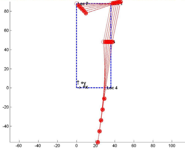
APG B2006, 5 Nov 2004, hammer impacts @ C; ODS for mean resonant frequency = 18.3429 Hz
