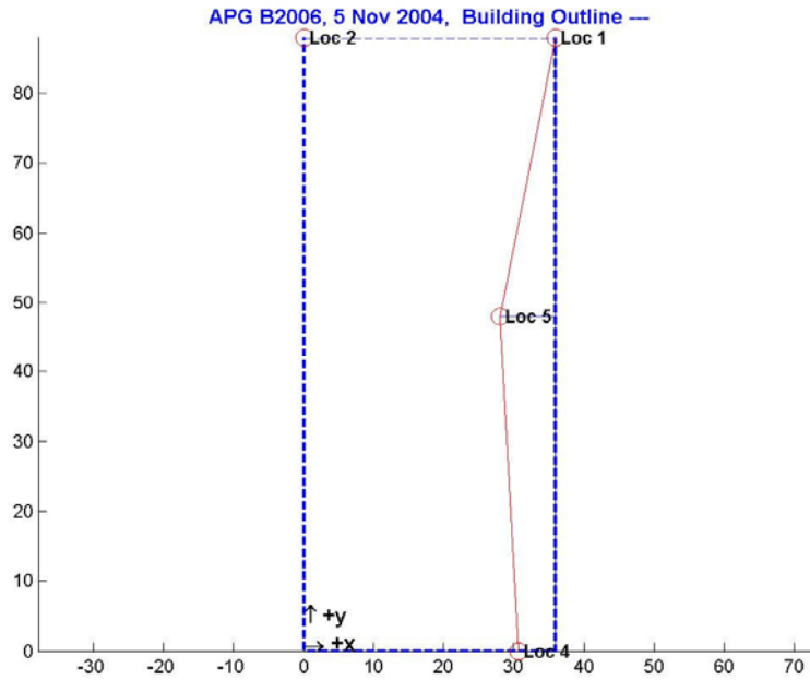
Figure 4-31. Undeformed Building Outline and Annotated Measurement Locations; x, y in feet
