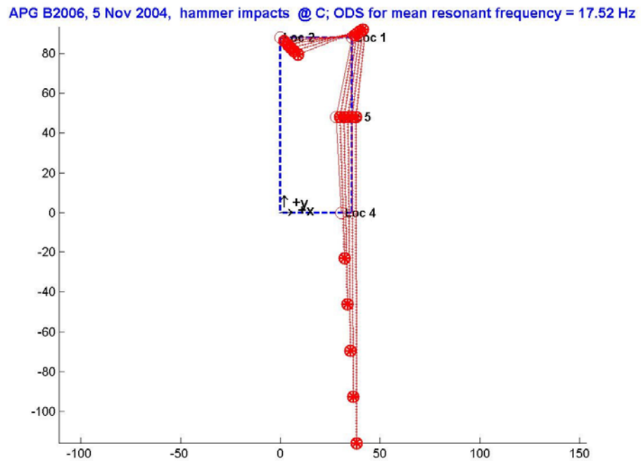
Figure 4-40. APG Building 2006 ODS Mode Shape Displayed Statically in Plan for 17.5 Hz; x, y in feet
