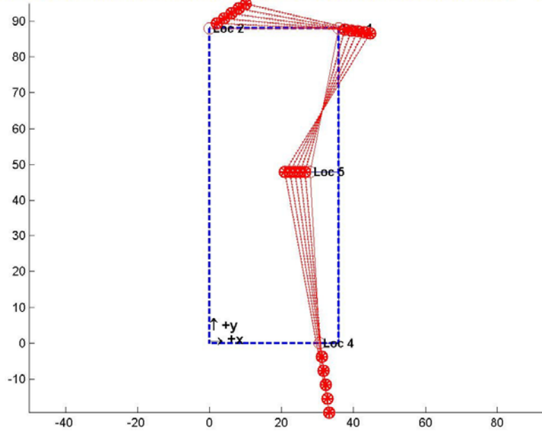
APG B2006, 5 Nov 2004, hammer impacts @ C; ODS for mean resonant frequency = 20.3029 Hz
