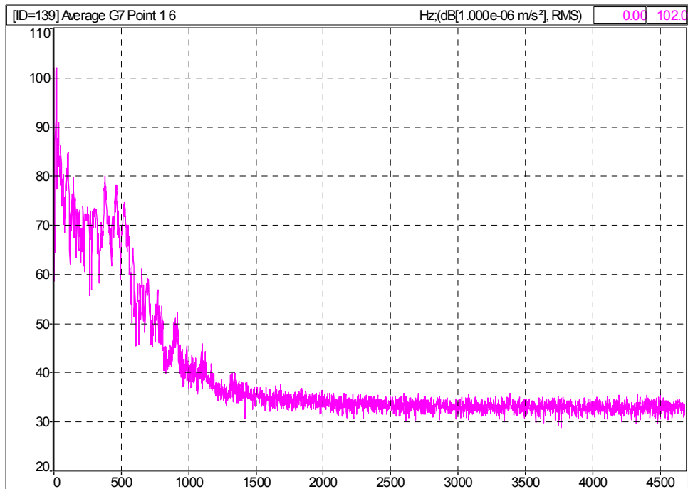
(b) Glass acceleration power spectrum, dB re: 1 \mu\text{m}/\text{sec}^2 rms, versus frequency, Hz
