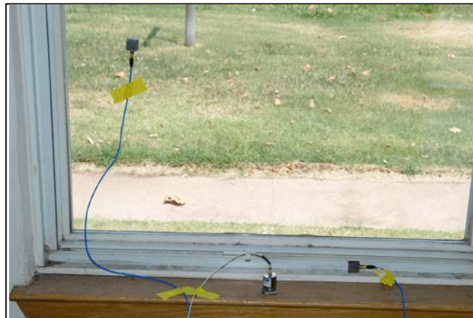
Figure 3-55. Accelerometer Placement On and Around Window, Building 6961B, Interior
