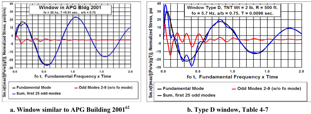
Figure 4-58. Time Histories of Stress Response to Blast for Two Windows
