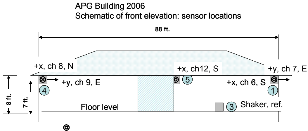
Figure 3-22. Plan Schematic Showing Numbered Locations and Orientations of Accelerometers
