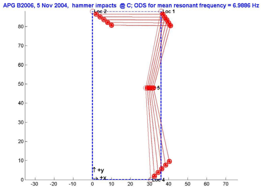
Figure 4-32. APG Building 2006 ODS Mode Shape Displayed Staticly in Plan for 6.99 Hz; x, y in feet
