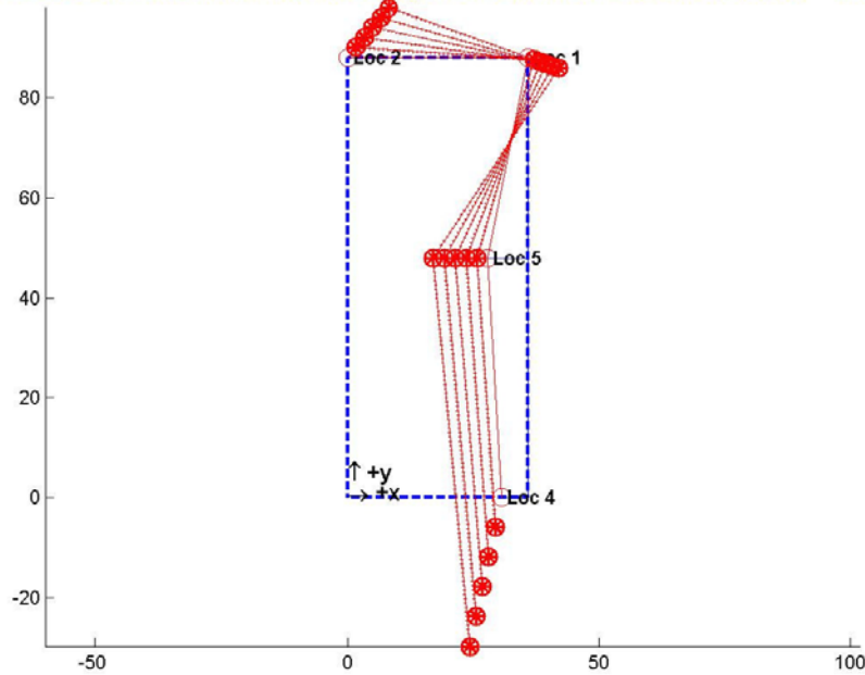
APG B2006, 5 Nov 2004, hammer impacts @ C; ODS for mean resonant frequency = 23.4857 Hz
