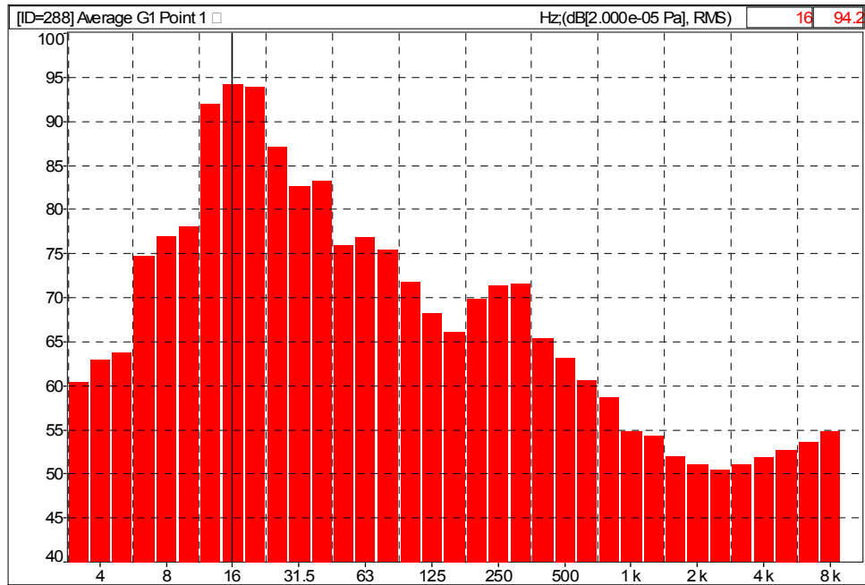
(a) Sound power spectrum, dB re 20 μPa rms versus band center frequency, Hz
