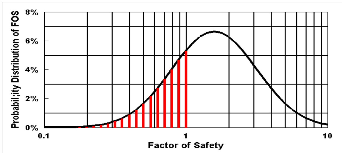
Figure 4-64. A Lognormal Distribution of the FOS; The log mean of the FOS is 1.6, the standard deviation of the log of the FOS is 0.3 and the POD is 28%
