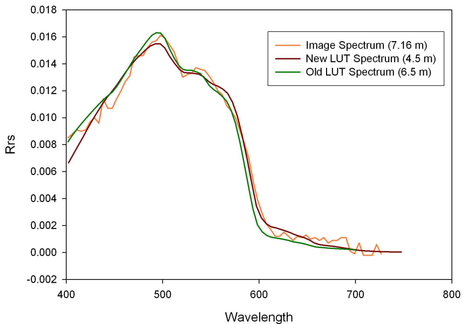
Figure 4. Image spectrum and the selected LUT spectra from plot position 1 in Figure 2. Note the note that the new LUT spectrum matches the Rrs spectra better than the old LUT. However, the new LUT has a greater bathymetric error.
