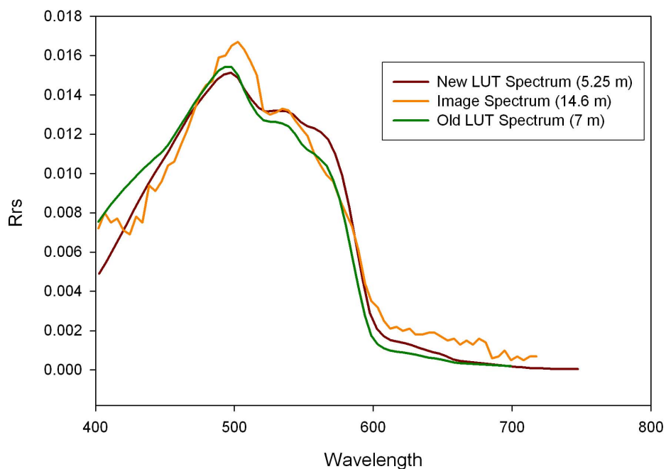
Figure 3. Image spectrum and the selected LUT spectra from plot position 1 in Figure 2. Note the note that the new LUT spectrum matches the Rrs spectra better than the old LUT. However, the new LUT has a greater bathymetric error.
