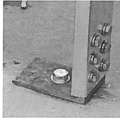
Figure 3. Stud-to-Floor Anchorage using a 1/2"-thick Steel Angle
