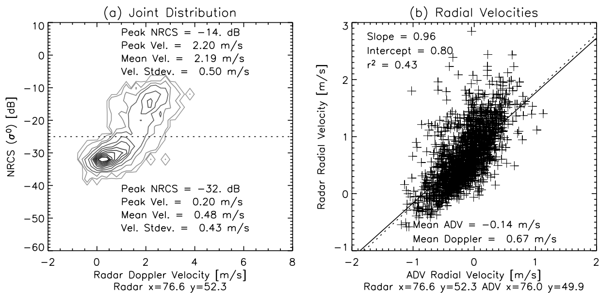
Figure 3: (a) Contour plot of joint histograms of NRCS and Doppler velocity for the time series shown in Figure 7 ( x=76.6 m, y=52.3 m). The NRCS bin size is 2 dB and the Doppler velocity bin size is 0.2 m/s. (b) Radar Doppler velocity versus ADV radial velocity. Doppler velocities were selected from pixels with NRCS value between -40 dB and -25 dB. The solid line shows the least squares fit for the data, and the dotted line is a one to one relationship with an 0.81 m/s offset.
