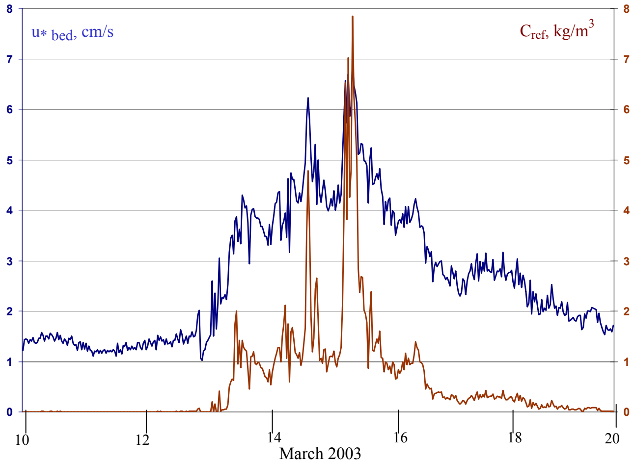
Figure 2. Bottom bed friction velocities (blue) and C_{ref} determined from combined wave-current bottom boundary layer model (Wiberg, et al., 1994). Input data for model was obtained with instrumented tripod.
