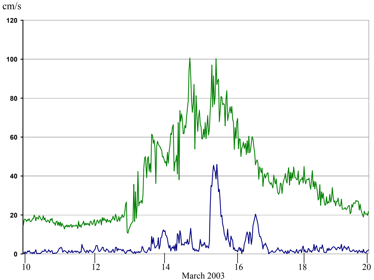
Figure 1. Bottom current speed (blue) and significant bottom wave speed (green) measured with the PC-ADP.
