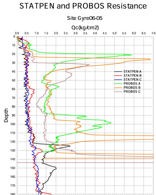
STATPEN and PROBOS Tip Resistance from Gyre 6, Site 5 plotted to same scale. Depth is relative to mudline. Peaks in the PROBOS data at about 30 cm depth are attributed to dilative behavior of granular layers at that depth.
