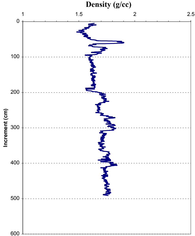
Figure 1. Multi-sensor whole core density log of piston core PCFL-665 showing several higher density zones indicative of debris flow deposits.
