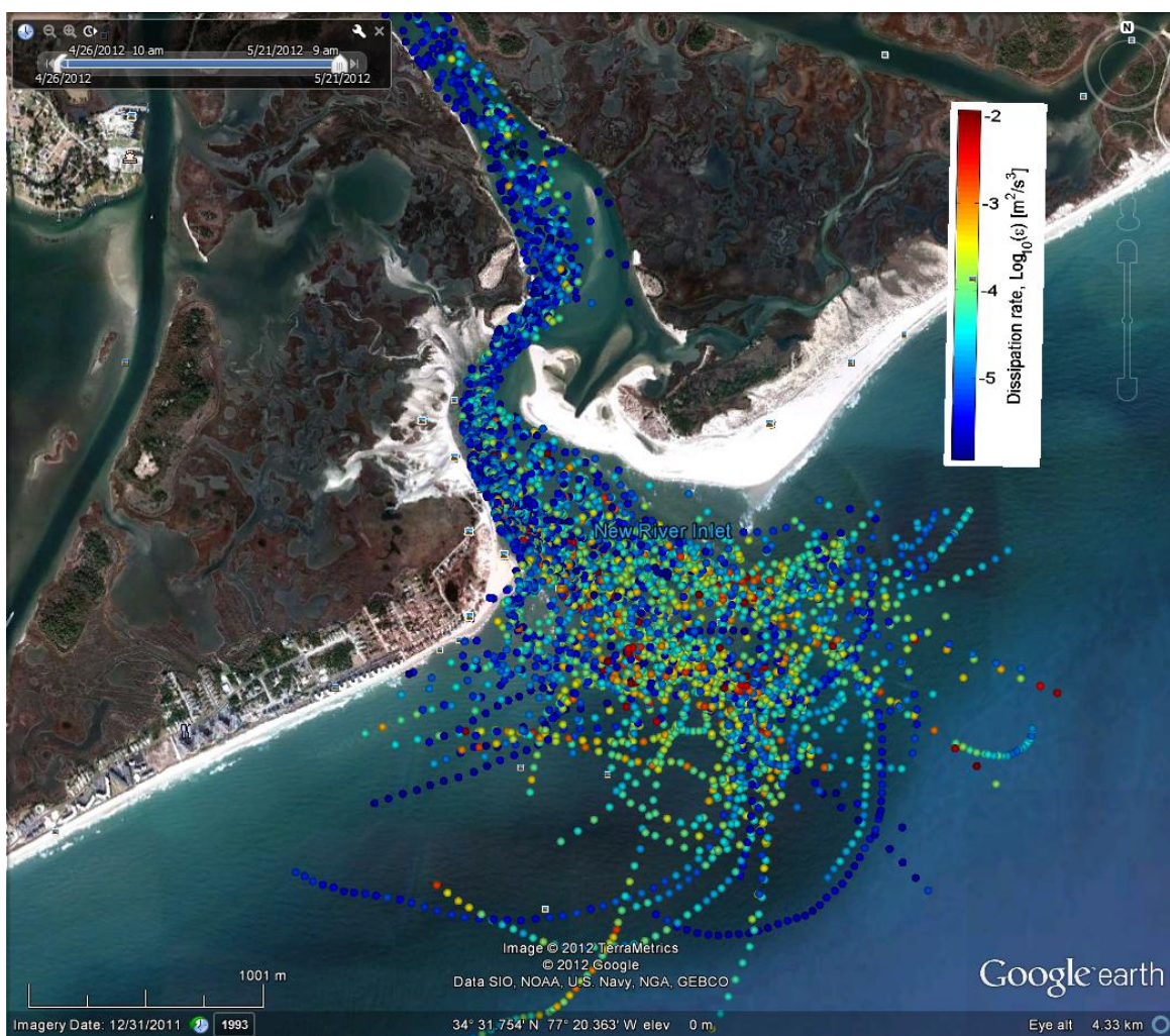
Figure E2. Aggregate SWIFT tracks from the month-long experiment at New River Inlet. Colors indicate surface dissipation rate (log scale).
