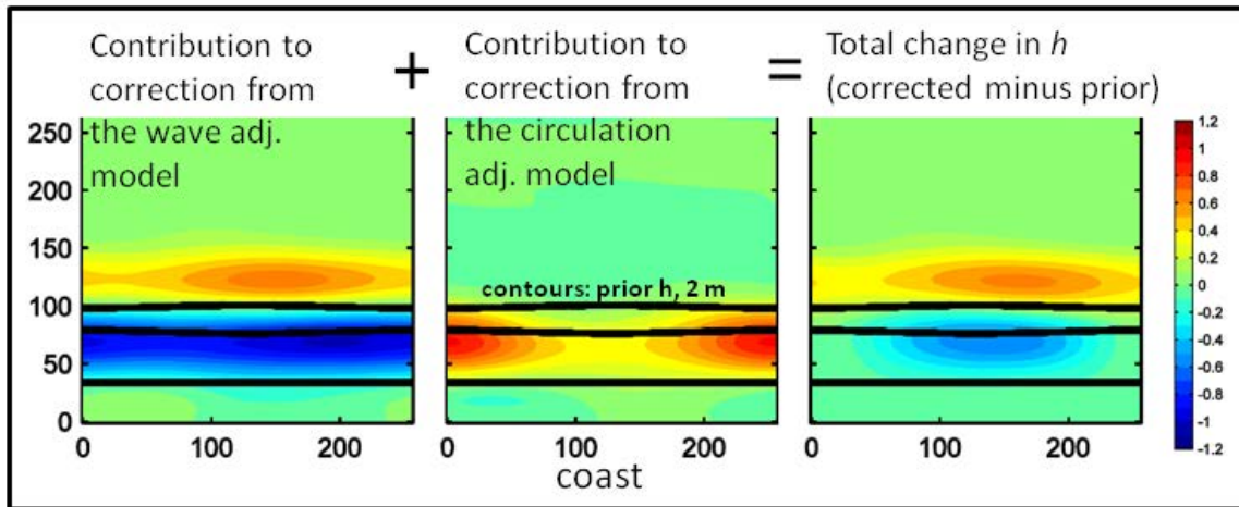
Figure G3: (from left to right) Contribution to the bathymetry correction by wave model, circulation model and both models. The wave model provides correction the bar location without any alongshore variability, whereas the circulation model provides an alongshore variable correction without changing the bar location.
