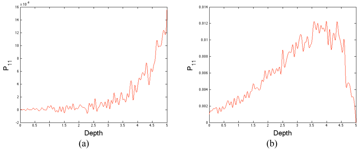
Fig. 8 Dependence of Scattering and Transmission part of radiance on depth (a) P_{11} at 0^\circ (scattering) (b) P_{11} at 180^\circ (transmission)
