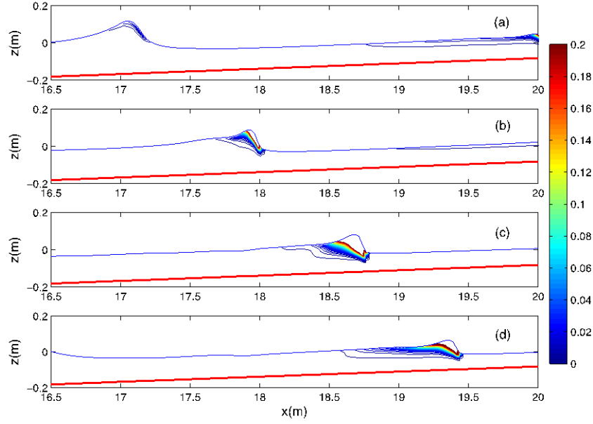
Figure 3. Void fraction distribution below progressive breaking wave crest in NHDAVE.
