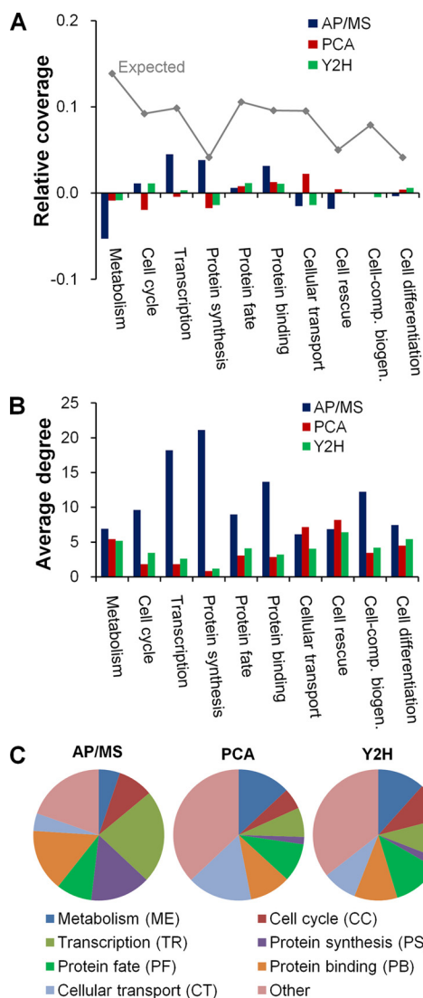
FIG. 1. Functional diversity among proteins and interactions present in the high-confidence data sets. A, The relative distribution of all proteins from Saccharomyces cerevisiae , as annotated according to the Munich Information Center for Protein Sequences functional categories, is shown by the gray line labeled “Expected.” It denotes the relative fraction (coverage) of all yeast proteins that belong to a given category. The deviations of the AP/MS, PCA, and Y2H high-confidence data sets from this distribution are shown by the different colored bars, e.g. proteins labeled “Metabolism” are relatively under-represented in the AP/MS data set. B, The average degree of the proteins in a given functional category for each high-confidence data set. C, The relative distribution of protein-protein interactions in the different functional categories for each high-confidence data set.
