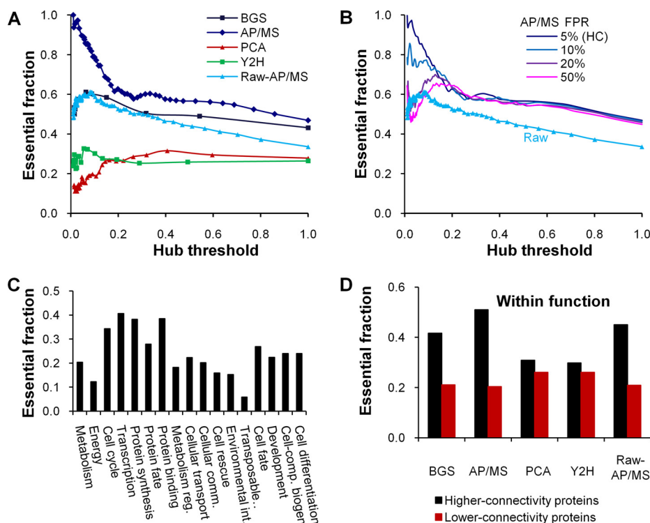
FIG. 8. Distribution of essential proteins. A, The fraction of essential proteins among hub proteins as a function of hub threshold, represented as the fraction of (hub) proteins with degrees larger than a given degree among all proteins of the studied protein interaction network. For example, a hub threshold of 0.1 means that we selected the highest top 10% connected proteins as hubs. B, The essential fraction of proteins in the AP/MS data are shown for several different false positive rates, indicating the sensitivity of the essentiality-connectivity correlation to the confidence level of the data. C, The fraction of all yeast proteins that were essential as a function of the Munich Information Center for Protein Sequences (MIPS) function categories. D, More connected proteins within the same MIPS function category tended to be essential for all five data sets. For each MIPS complex, we calculated the average degree and extracted proteins of above-average degrees ( Higher-connectivity proteins ) into a group and those with below-average degrees ( Lower-connectivity proteins ) into another group. After scanning all MIPS complexes, we calculated the fraction of essential proteins in each group. The consensus conclusion indicated that higher-connectivity proteins were indeed more essential than lower-connectivity ones.
