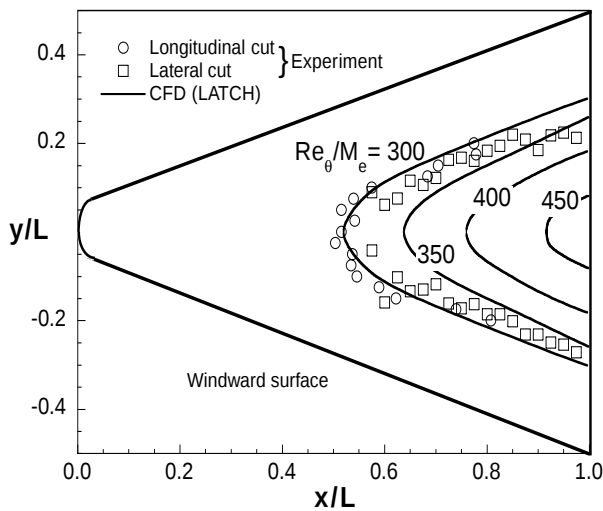
b) Correlation with Re_{\theta}/M_e parameter
