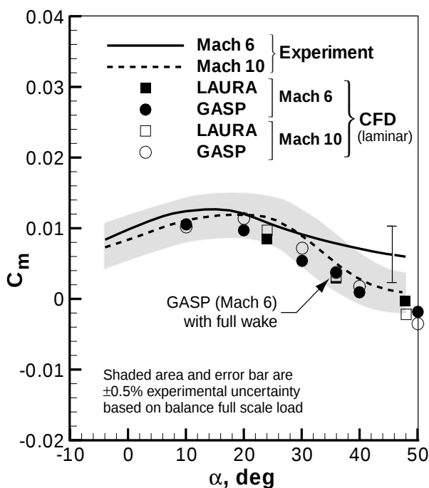
Figure 7. Comparison of measured and predicted pitching moment (baseline). (adapted from Murphy, et al. [23]).
