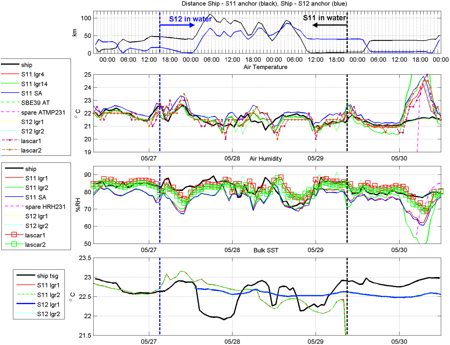
Figure 3-7. Comparison between ship measurements adjusted to buoy height (2.9m for ATMP, HRH, BPR and 3.3m for WSPD) and data from Stratus 11 and 12. Distance between R/V Melville and buoy anchor positions (top), air temperature and relative humidity (center), bulk SST (bottom).
