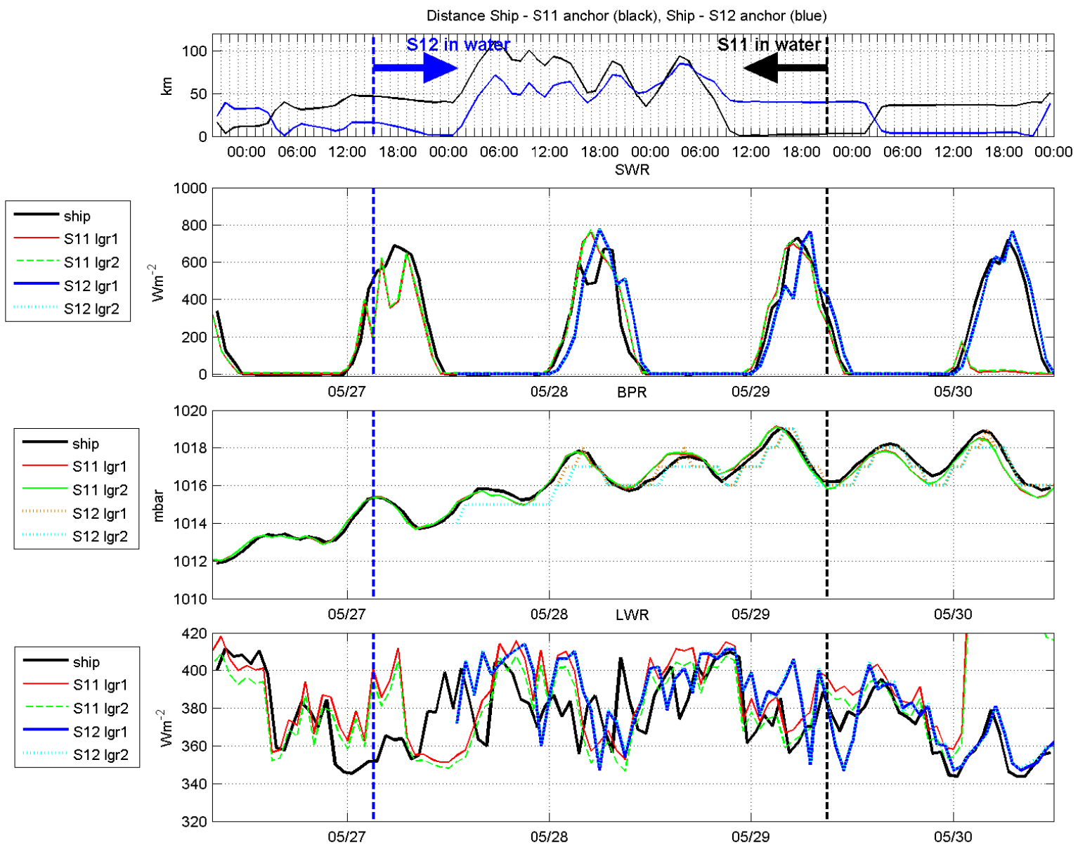
Figure 3-8. Same as Fig 3-7 but for shortwave (SWR), barometric pressure (BPR) and longwave (LWR).
