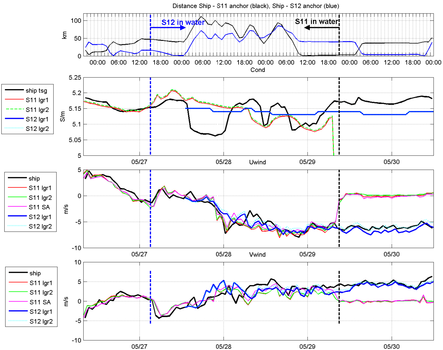
Figure 3-9. Same as Fig 3-7 but for near-surface conductivity, eastward wind speed, northward wind speed.
