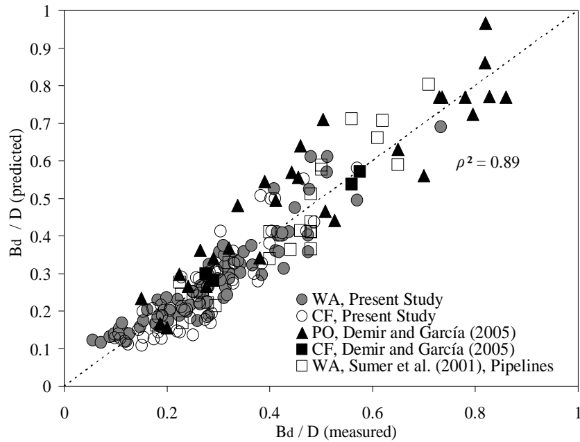
Fig. 4. Measured final relative burial depth from the present study and from other researchers. Predicted values are obtained by using Eq. 1.
