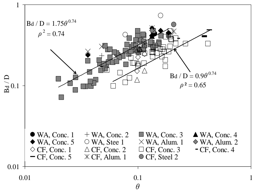
Fig. 2. Equilibrium burial depth as a function of the Shields Parameter \theta . Experiments conducted in the wave flume.
