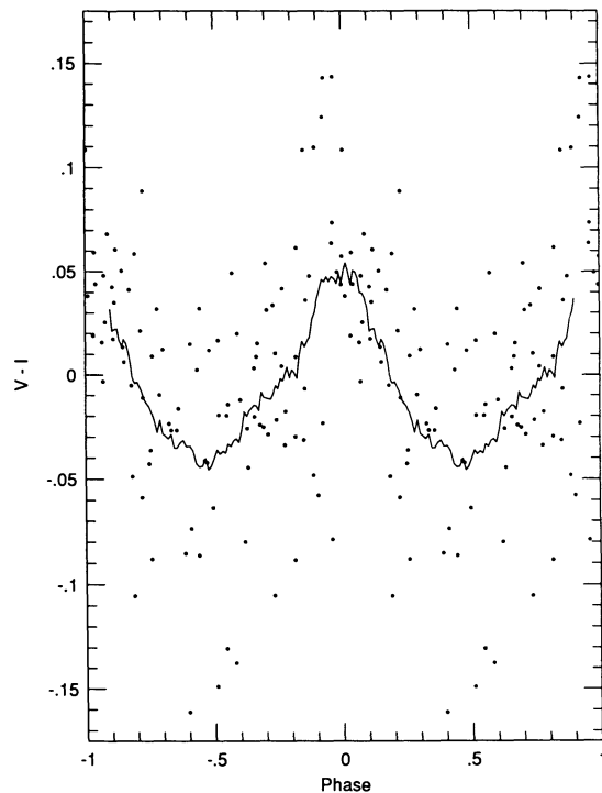
FIG. 3.—Normalized instrumental V-I light curve vs. photometric phase as determined from eq. (1). The normalization was performed in the same manner as Fig. 1. A single point is the result of a single I-V-I combination where the I -values were averaged. The rms scatter for a single point is \pm 0.08 mag and was determined from the first differences of the magnitudes sorted by phase. The phase sorted data was smoothed by generating a running mean using 20 points and is indicated by the line. Two full cycles are shown.
