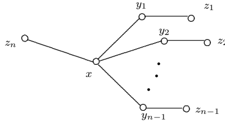
Figure 2: The graph G
