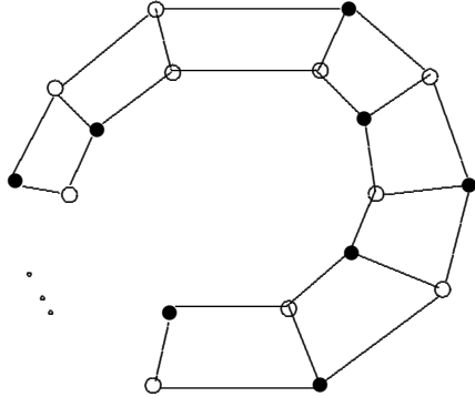
Figure 4: The independent set for the prism C_n \times K_2
