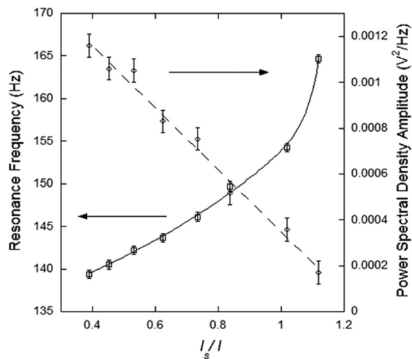
FIG. 3. The change in resonance frequency and peak amplitude in the power spectrum at this frequency measured in an AC field of 0.0162 Oe as a function of the inverse length l of the wire used to suspend the weight. The cantilever length l_s is 5 cm and tensile force is 1 N.
