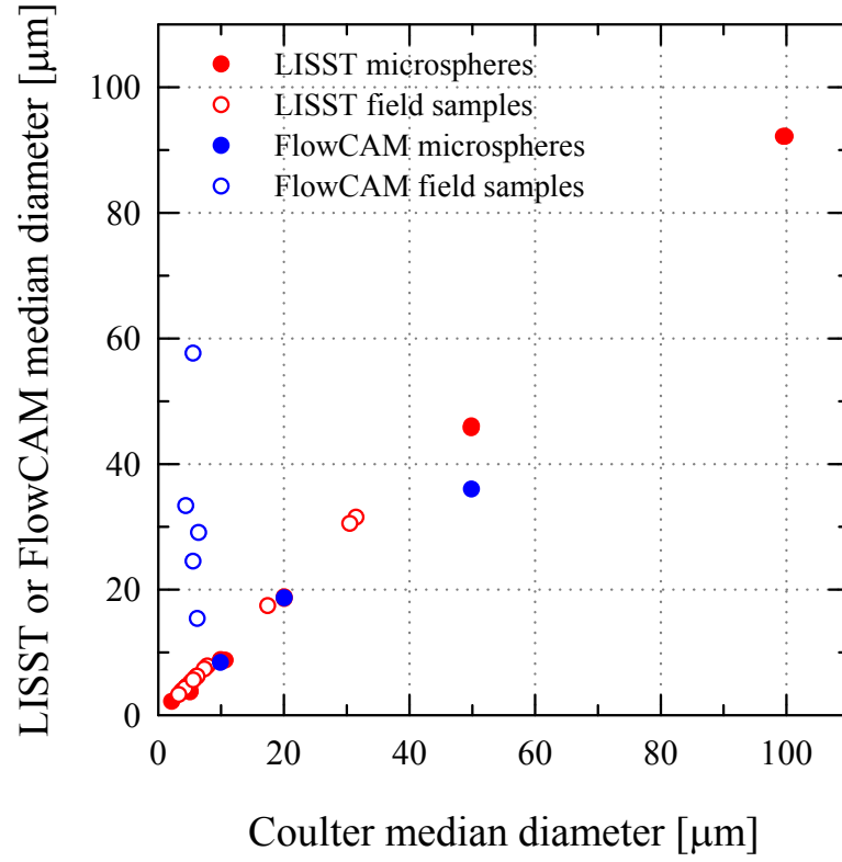
Figure 3. Scatter plot comparing the median particle diameter derived from particle volume distributions measured with the Coulter counter, LISST-100X, and FlowCAM. Experiments include monodisperse suspensions of polystyrene microspheres of varying size (filled symbols), and natural seawater samples collected from the field (open symbols).
