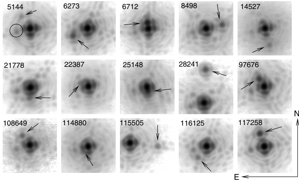
Figure 1. Images of some resolved close companions in the red channel ( 2.272\ \mu\text{m} ), marked by with the HIP numbers. Negative logarithmic intensity scale from 10^{-3} to maximum, each fragment is 50 \times 50 pixels ( 0''.9 ). The prominent “ghost” companion to the left of each target (circled in the first image) is a reflex in the NICI optics.
