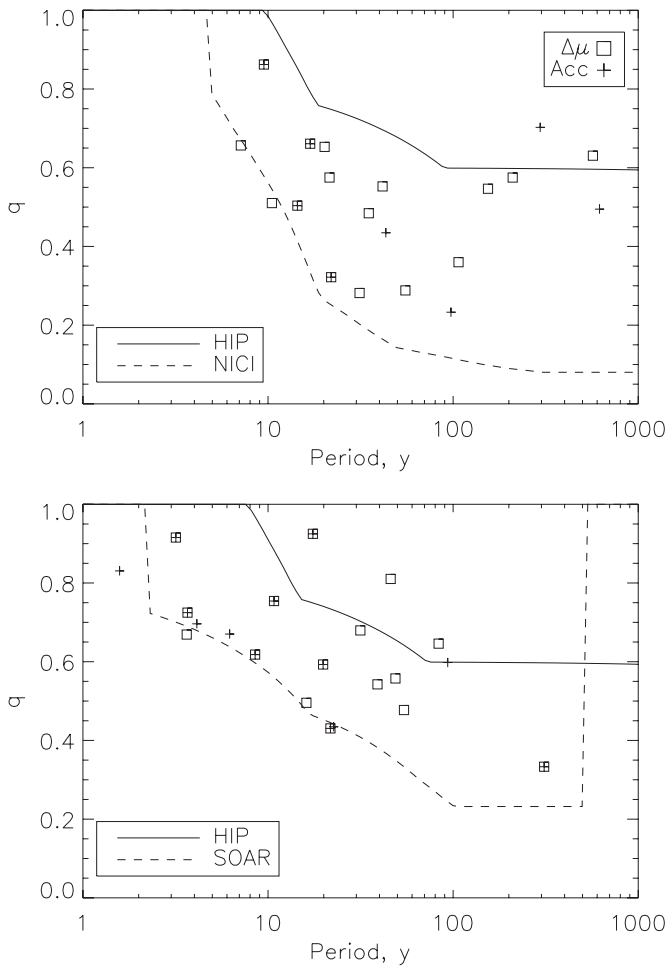
Figure 3. Astrometric binaries from FG-67pc actually resolved with NICI (top) and speckle (bottom) in the (P, q) plane. Squares and pluses mark \Delta\mu and \dot{\mu} binaries from MK05, respectively. The curves indicate approximate detection limits at 50 pc distance.
