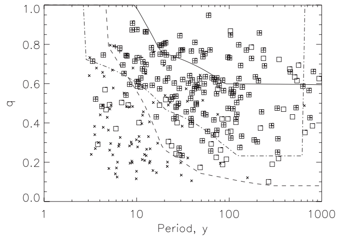
Figure 6. Simulated direct resolution of 353 astrometric binaries by NICI (squares, N = 195 ) and speckle (pluses, N = 151 ). Unresolved objects are plotted as small crosses. The curves indicate approximate limits of direct resolution with Hipparcos (full line), NICI (dashed line), and speckle (dash-dot line) for binaries at 50 pc.
