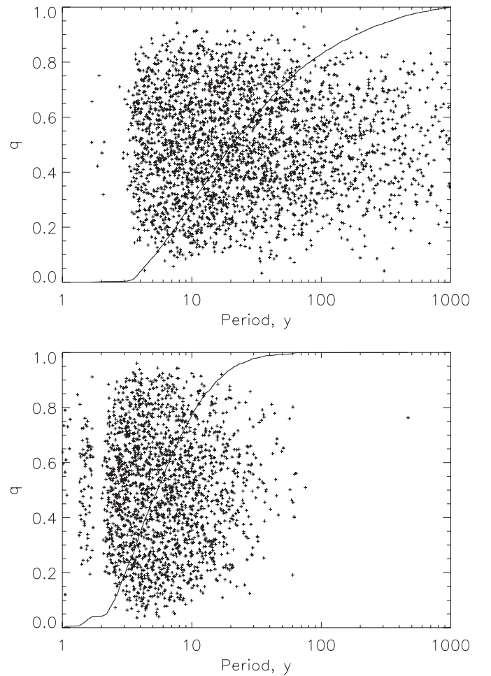
Figure 4. Distributions of simulated \Delta\mu (top) and \dot{\mu} (bottom) binaries in the (P, q) parameter space. The curves indicate cumulative period distributions. Binaries with log-uniform period distribution were simulated in this case.
