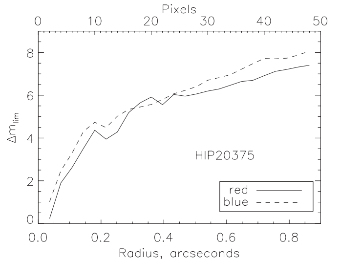
Figure 2. Limiting magnitude difference for companion detection in the red (full line) and blue (dashed line) channels for HIP 20375, a typical case with Strehl ratio of 0.40 in the red channel.
