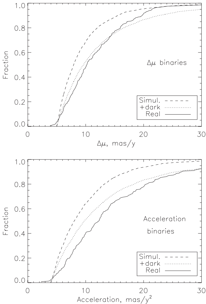
Figure 5. Cumulative distributions of simulated and real astrometric binaries. The simulations are performed assuming either only red dwarf companions (dashed lines) or a certain fraction of dark and massive companions (dotted lines). Top: distribution of \Delta\mu . Bottom: distribution of \mu .
