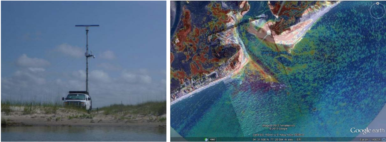
Figure 1. Left Panel: The Scripps self-contained X-band marine radar system mounted on a 4-wheel drive van supported “off grid” unique backscatter measurements at the New River Inlet. Right Panel: Overlay of radar backscatter with background satellite image (Google) and H hyperspectral overlay image collected by F.Feddersen on 5/8/2012.
