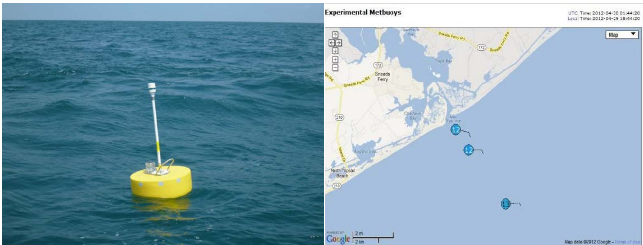
Figure 3. Left Panel: Deployed meteorological buoys measured wind speed/direction, GPS, air and sea temperature. Right Panel: Buoys deployed in cross-shore array, with shoreline values measured at radar site.
