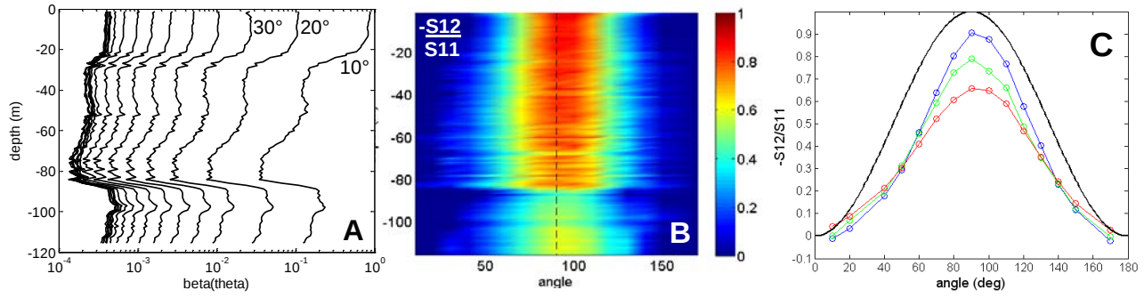
Figure 1. (A) Vertical profile of the VSF resolved from 10 to 170° in 10° increments collected in Santa Barbara Channel. (B) The linear degree of polarization ( -S_{12}/S_{11} ) as a function of depth and angle, showing a maximum around 0.9 at the very surface, with a steady decrease with depth. The deep scattering maximum exhibited much lower polarization, as low as 0.6 around 90 m. (C) Overlays of -S_{12}/S_{11} plotted for 3 depths regions, labeled in B. This is the first time these measurements have been made in-situ.
