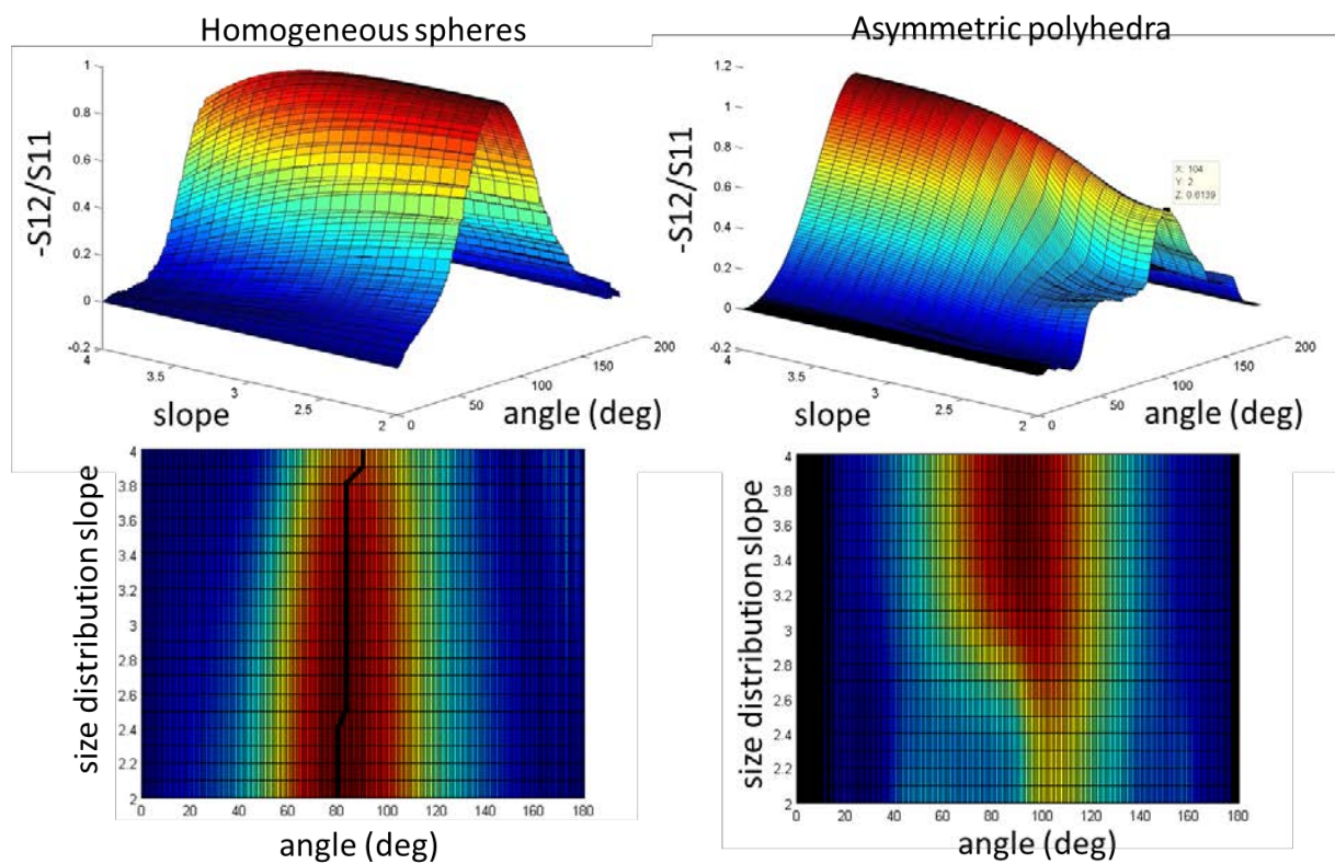
Figure 4. Same as in Fig. 2, with real refractive index, n_p = 1.20 .
