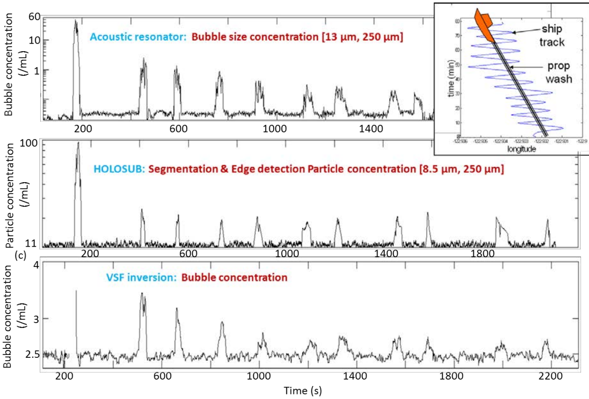
Figure 6. Bubbles resolved in a boat's propeller wash with an acoustic resonator (Czerski, Vagle), a holographic imaging system (Talapatra, Katz, Twardowski, Sullivan), and inversion of the volume scattering function. Inset in the upper right shows the ship tract over time. Bubbles persisted for over 1 hour in surface waters after the boat passed, indicating stabilization by organic surfactants.
