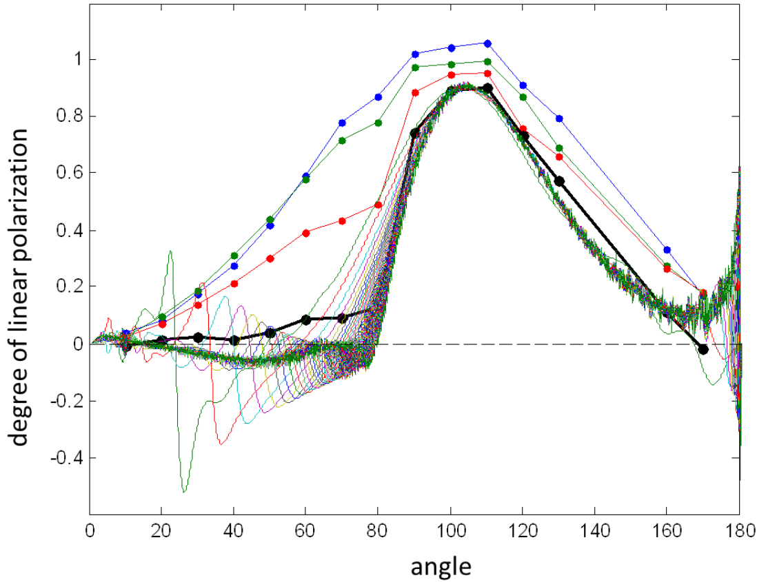
Figure 5. Degree of linear polarization ( -S_{12}/S_{11} from the Mueller scattering matrix) measured in the NY bight under breaking wave conditions (blue, red, green, and black traces), along with DOLP computed from Mie theory for various lognormally distributed populations of bubbles with relative refractive index of 0.75. A transition is observed between the background with little influence from bubbles (blue trace) to a particle population dominated by bubbles that matches Mie theory computations exceedingly well (black trace). In complex oceanic particle populations, the DOLP for bubbles is completely unique.
