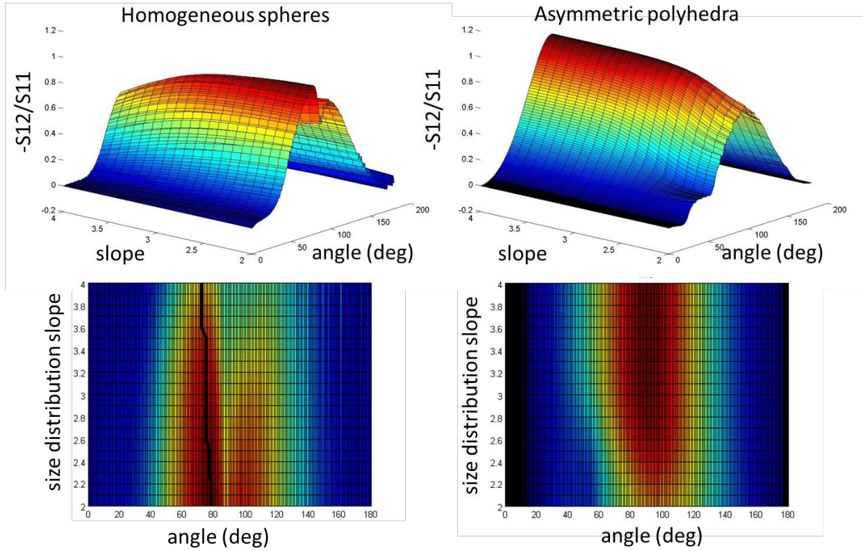
Figure 3. Same as in Fig. 2, with real refractive index, n_p = 1.10 .
