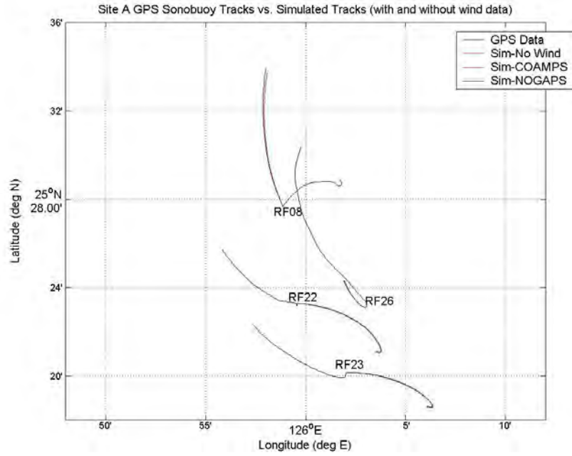
Figure 8: SFDM simulations results comparing no wind, with COAMP wind data and with NOGAPS wind data to the GPS data from sonobuoys at LWAD site A.
