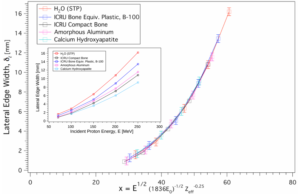
Figure III.3 Universal scaling of the lateral edge width (lateral penumbra). Phantom configuration is the same as for data in figure 2. Note that the exponent for Z_{\text{eff}} is 1/4 rather than 1/3 found for the distal edge width. The inset shows the unscaled lateral edge width for comparison.
