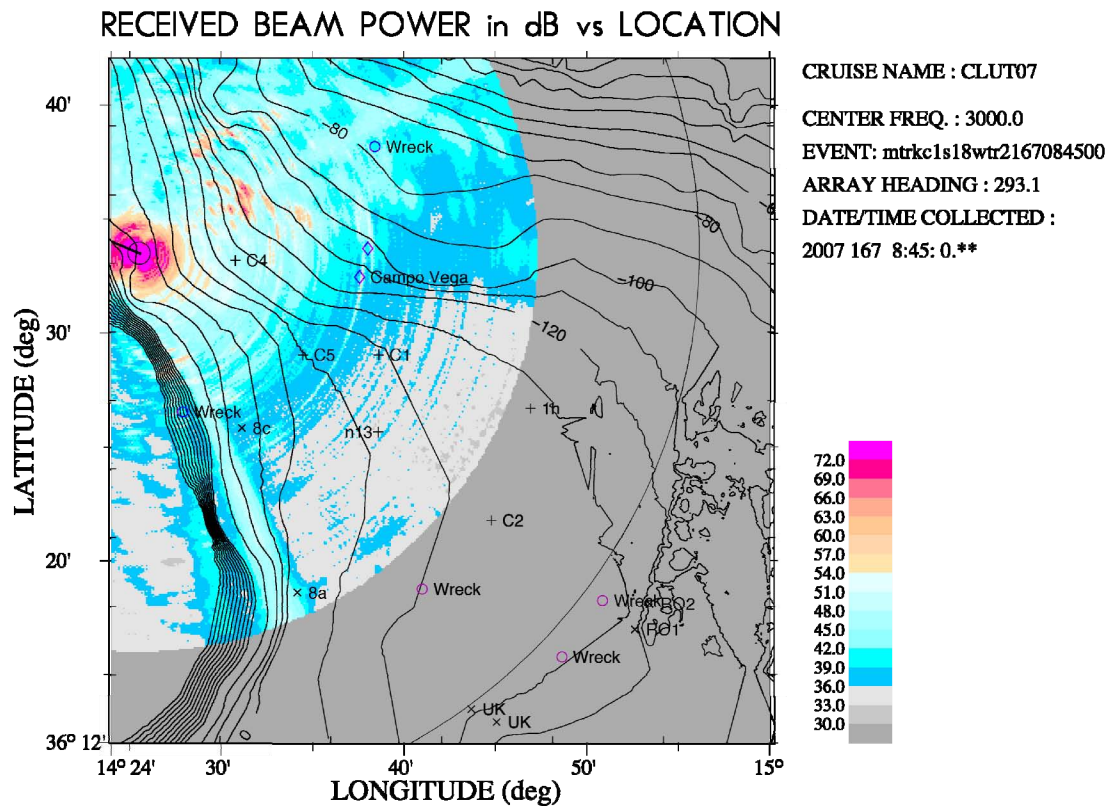
Fig. 1. Polar plot of the bistatic reverberation on the FORA cardioid array from a 1s LFM pulse on the Malta Plateau in the 2500–3500 Hz band. Levels indicated by color scale are in dB//1μPa 2 /Hz. The array heading is 293°T. Left-right ambiguity is broken by the cardioid beamformer and shows excellent left-right rejection on various clutter features (most likely carbonate mounds and mud volcanoes).
