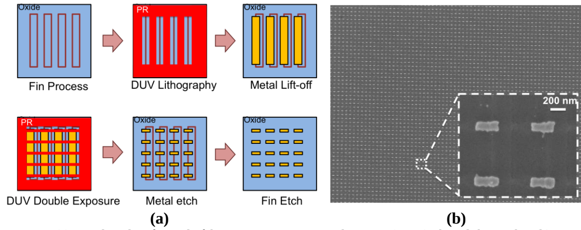
Figure 7. (a) Developed wafer-scale fabrication process using deep-UV (DUV) photo lithography. (b) SEM picture of the large area optical antenna array fabricated on 6 inch wafer.
