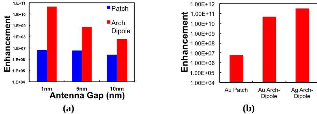
Figure 4. (a) Field enhancement comparison between patch antenna and arch-dipole antenna. Field enhancement of arch-dipole keeps increasing with antenna gap scaling down. (b) Field enhancement comparison of 1 nm gap gold patch antenna, gold arch-dipole antenna and silver arch-dipole antennas. (FDTD simulations)
