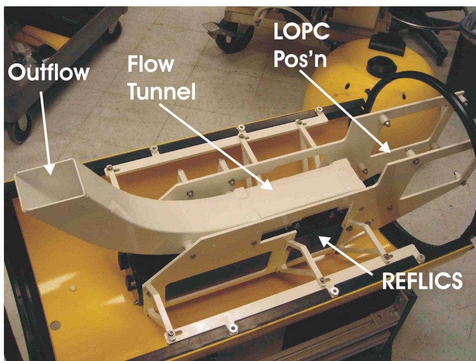
Figure 4. Photograph of flow assembly to hold LOPC and REFLICS in MBARI's Dorado AUV. [The upper half of the cylindrical, 53-cm-diameter outer casing of the AUV payload section is shown with the flow channel exposed. Flow enters the front of the AUV on the right, passes in its entirety through the LOPC sample tunnel, and in part through the REFLICS sample volume, before exiting the sample tunnel through the outflow port. The nose cone is shown in the background, with rectangular port.]
