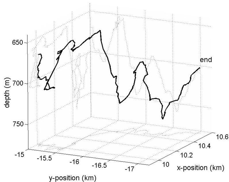
Figure 1. Three dimensional track of a sperm whale localized using the DRTD method and 5 bottom-mounted hydrophones in the AUTECH range. The track represents 25 minutes of data. Projections onto the three planes are shown with dotted lines.
