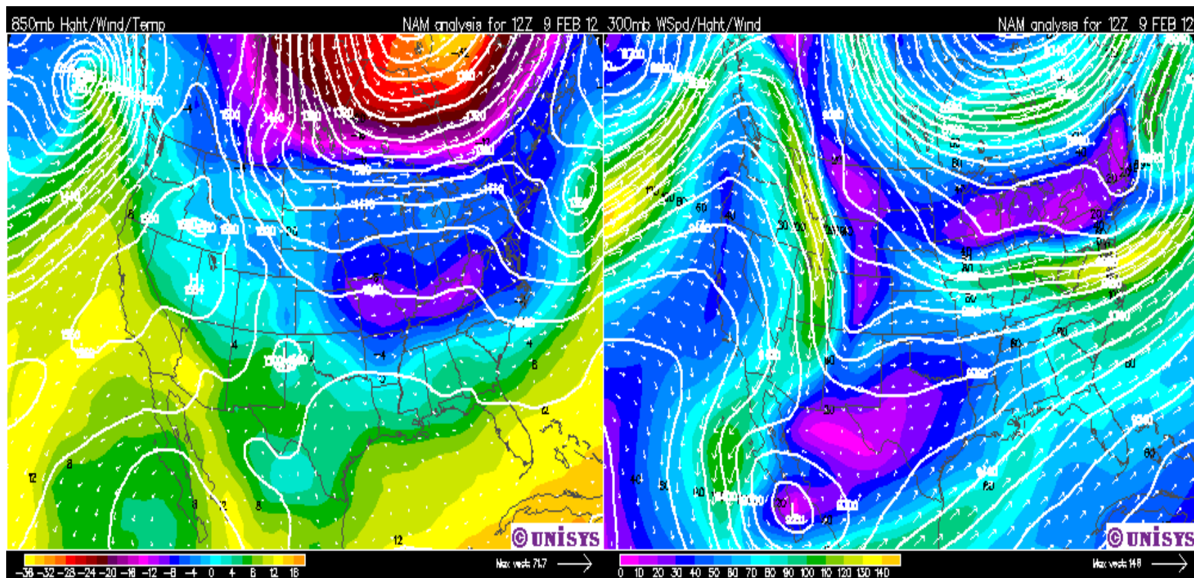
Figure 2. The 850 hPa and 300 hPa analysis charts for 1200 UTC, February 9, 2012.
