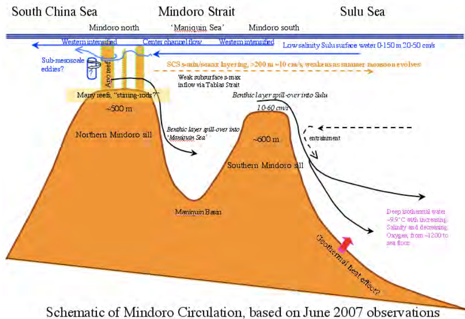
Figure 6. Mindoro Strait Schematic of along-axis summer monsoon circulation and stratification, as determined by the observed thermohaline stratification and shear.
