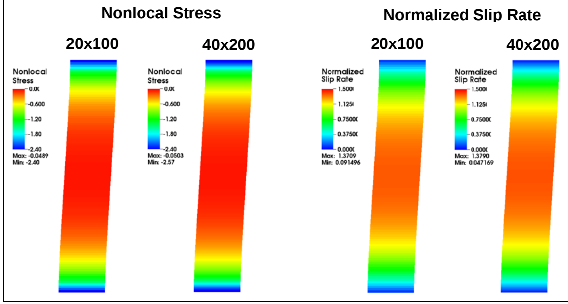
Figure 5. Comparison of nonlocal stress and the slip rate for the 20x100 and 40x200 element simulations of the 5- \mu\text{m} -thick single crystal. The results are shown at a 0.05 shear strain.
