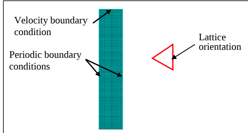
Figure 1. Initial configuration for the single crystal and the crystal lattice orientation. The bottom is fixed and the top is moved to the right. Periodic boundary conditions are applied coupling the left and right hand sides.
