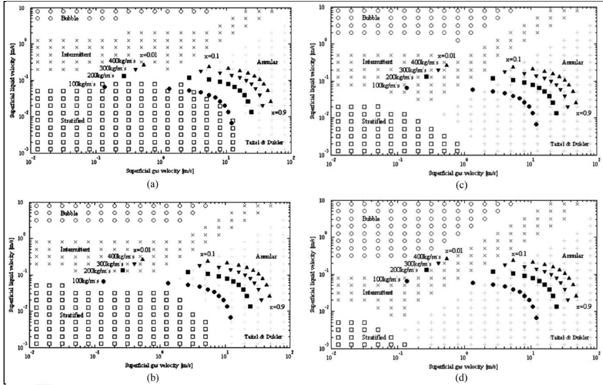
Figure 5. Taitel-Dukler flow regime maps for R13 flowing in a horizontal channel of various diameters (a) 100 mm, (b) 10 mm, (c) 1 mm, and (d) 0.1 mm (28).
