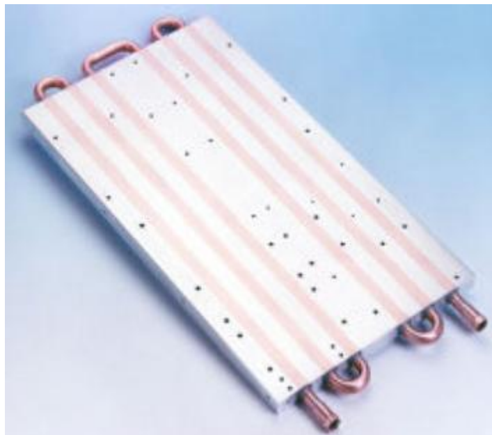
Figure 3. Hydroblok pressure-fit 6-pass serpentine cold plate (9).
