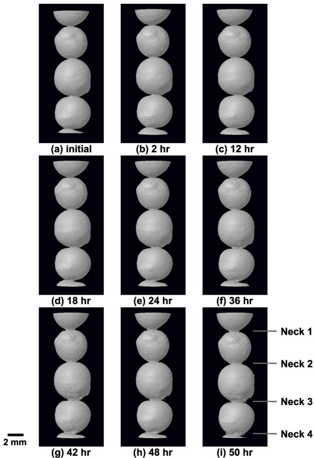
Figure 5. 3-D micro-CT images showing the structural changes of a 1-D ice sphere array maintained at -2.3 \pm 0.2^\circ\text{C} for 50 hours. The images were acquired using a 15\ \mu\text{m} image pixel size.
