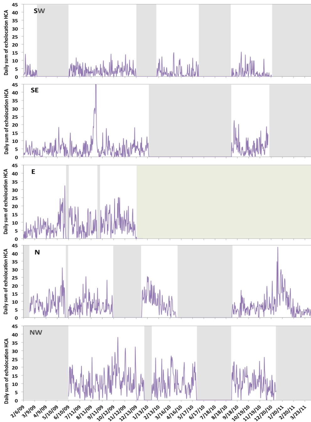
Figure 14. Occurrence of echolocation signals at the five deployment locations over the study period. Note: grey areas represent gaps in the data sets. The green area represents data periods that have not yet been analyzed.
