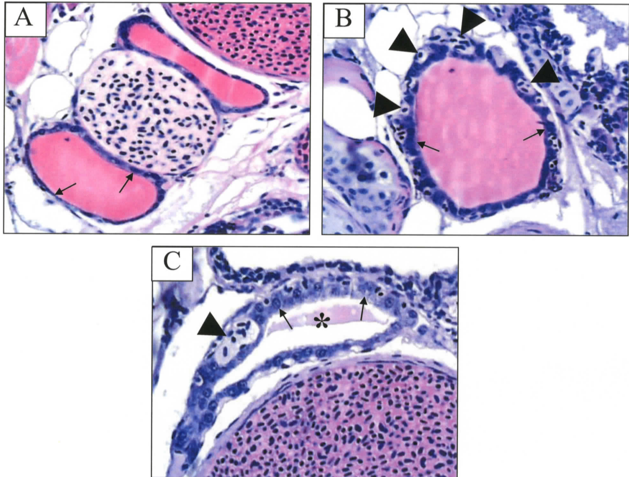
Figure 1. Photomicrographs of thyroid follicles of zebrafish reared in control water (A) or in water containing AP-derived perchlorate at measured concentrations of 11480 ppb for 12 weeks (B-C). Note the squamous epithelial cell layer in control fish (A, arrows), and the cuboidal-to-columnar shape of the cells in fish exposed to perchlorate (B-C, arrows). The follicles of perchlorate-exposed fish also contained higher numbers of blood vessels within the epithelial layer (B-C, arrowheads), and some follicles in these fish also showed signs of colloid depletion (C, asterisk). Hematoxylin-eosin stain. All photographs were taken at the same original magnification (x 100).
