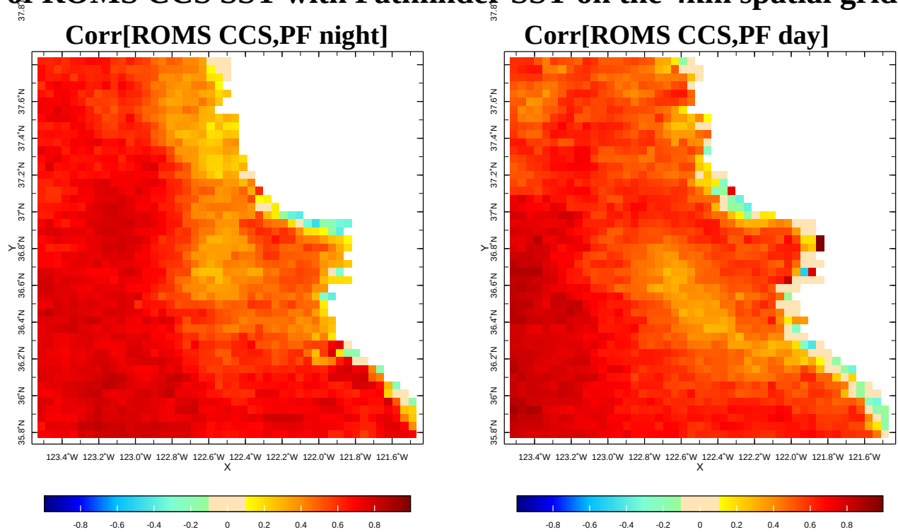
Figure 5. Correlation coefficients between daily values of ROMS CCS SST with Pathfinder SST for (left) nighttime and (right) daytime products, computed for year 2000 on the 4km spatial grid.
