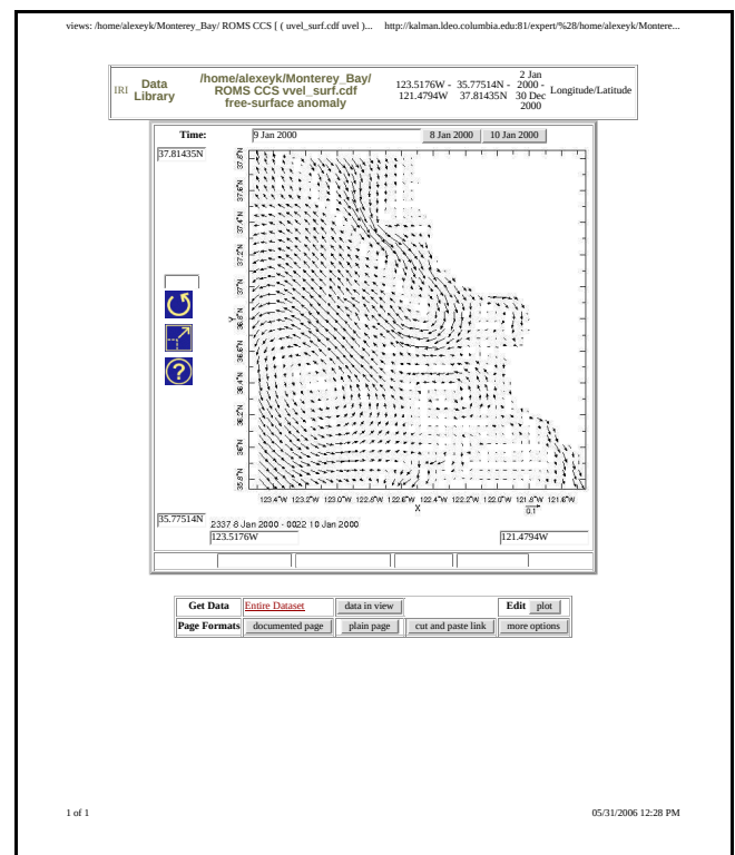
Figure 1. Visualization examples for Pathfinder SST and CCS surface velocity vectors via our Ingrid-based Data Catalog providing the access to selected Monterey Bay area data at http://rainbow.ldeo.columbia.edu/~alexeyk/Monterey_Bay.html
