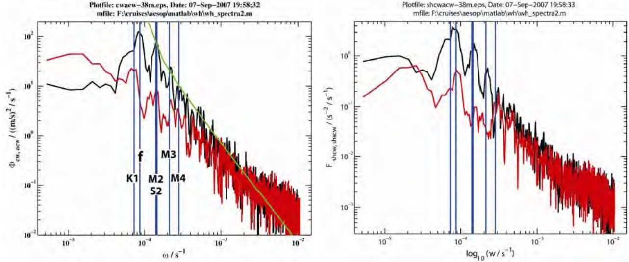
Fig. 3. Spectra of velocity (left) and shear (right) for the Workhorse bin 38 m above the bottom. Clockwise (anti-cyclonic) and Anti-clockwise (cyclonic) components are black and red. Vertical blue lines mark frequencies of K1, M2-S2, M3 and M4 tidal constituents as well as the near-inertial frequency, f . The data record is too short to separate M2 and S2. The green line is the modification of the Garrett-Munk internal wave continuum spectrum by Levine (2002). About 80% of the shear variance is in the discrete spectral lines.
