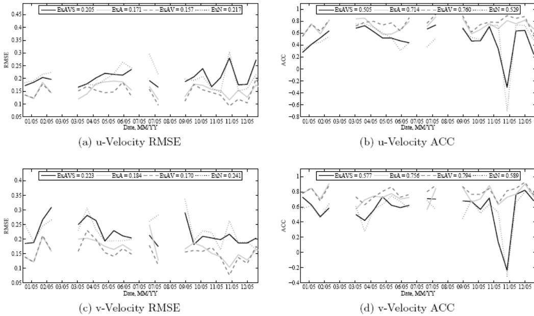
Figure 5: Timeseries of the root mean square error (RMSE) and the anomaly correlation (ACC) between the model and observations for zonal and meridional velocity for experiments ExN and ExAV.
