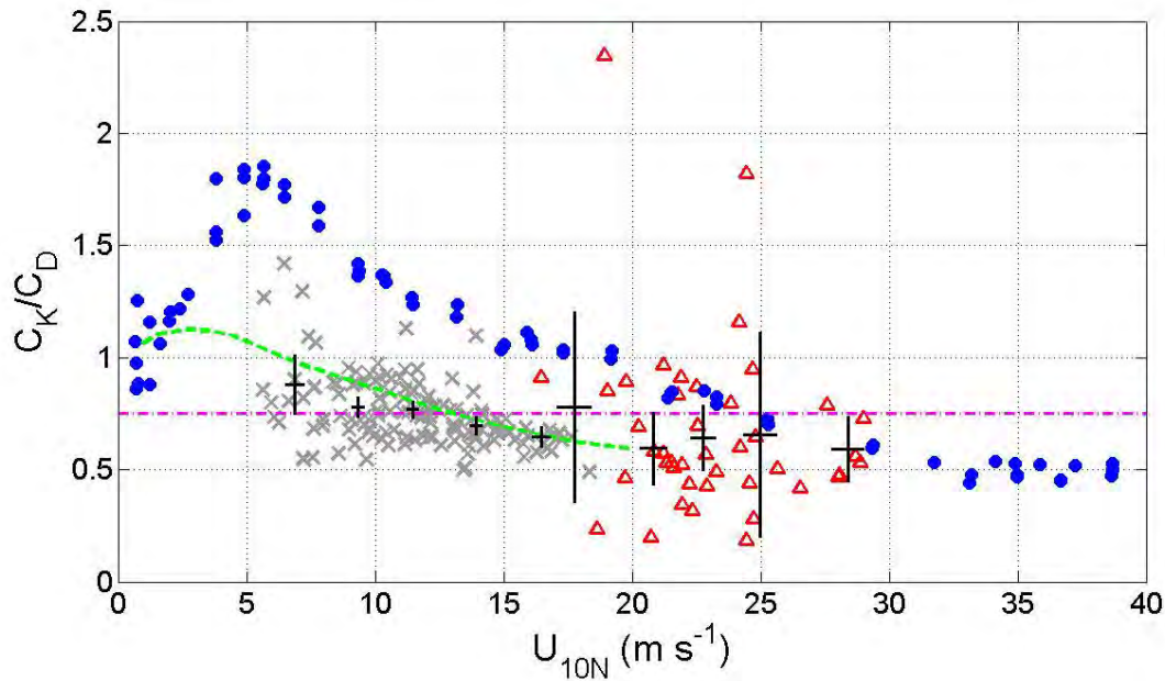
Figure 3. Wind speed dependence of C_K/C_D total heat exchange coefficient. ASIST laboratory results (●) and CBLAST ( \Delta ) measurements shown with HEXOS results (x). After binning observations by wind speed, the mean and 95% confidence intervals as determined from a t -distribution of the combined HEXOS and CBLAST field data are shown in black. Revised COARE15 relationship is shown (---), along with the threshold value of 0.75 suggested by Emanuel (1995).
