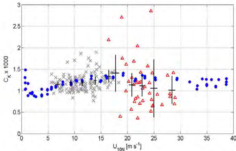
Figure 2. (Left) Wind speed dependence of total heat exchange coefficient. ASIST laboratory results (●) and CBLAST (Δ) measurements shown with HEXOS results (×). After binning observations by wind speed the mean and 95% confidence intervals of the combined HEXOS and CBLAST field data are shown in black.
