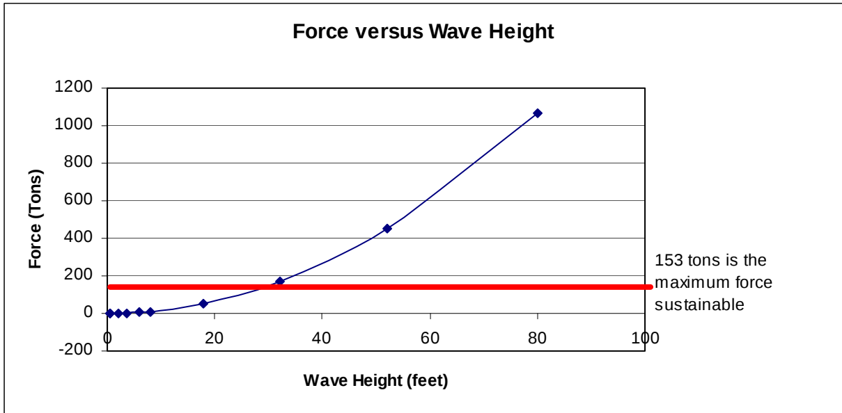
Figure 8: Comparison of Wave Energy to Rollover Force;
