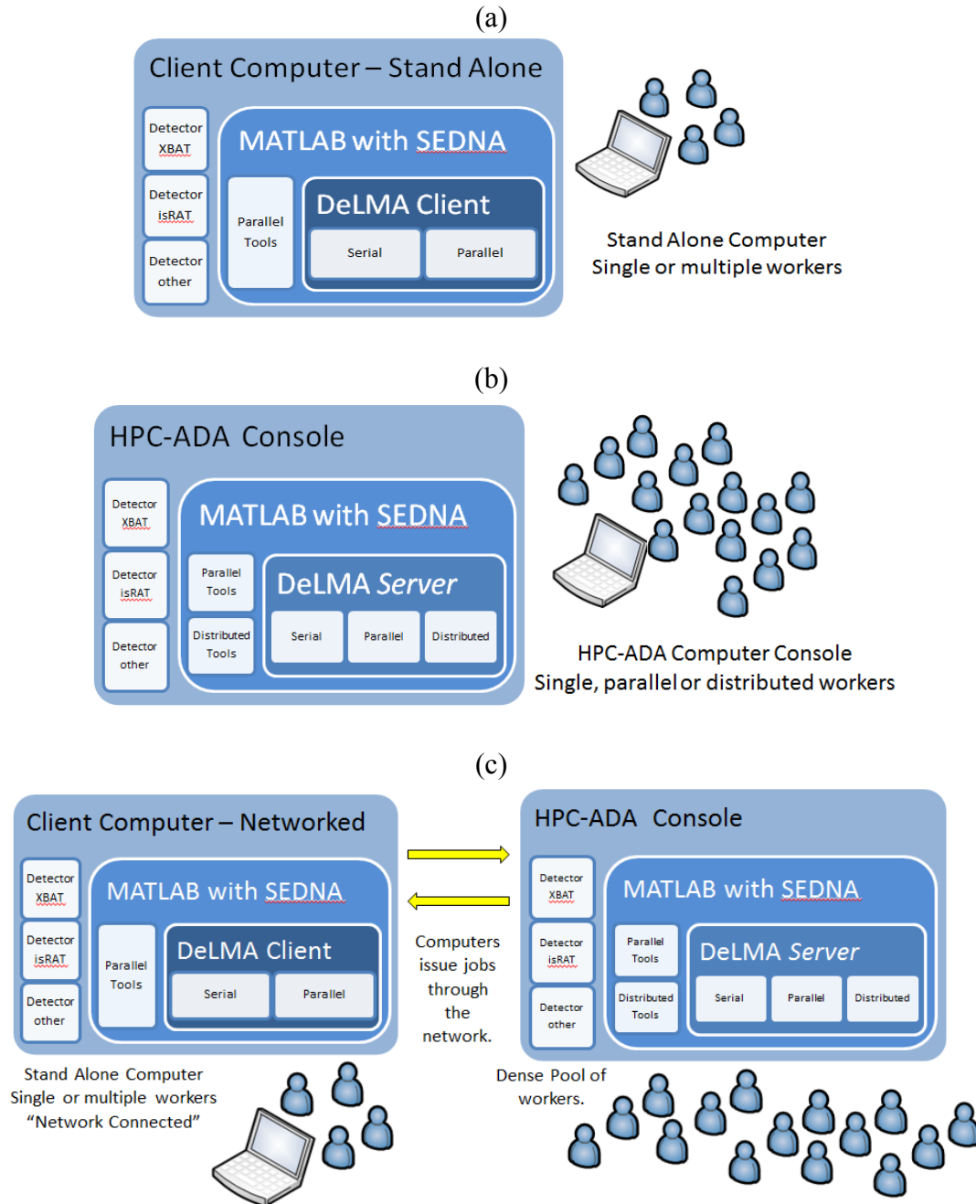
Figure 4. Figure shows three different configurations for parallel distributed computing referred to as Case 1, 2 and 3. This research uses the DeLMA software developed by Cornell University to realize each configuration. An embarrassingly parallel model allows standard detection algorithms to be added to the system, each will taking advantage of the parallel-distributed workers. (a) Case 1: Standalone mode, (b) Case 2: HPC-ADA console, serial, parallel or distributed and (c) Case 3: networked client-server model, opening up the HPC-ADA as a network appliance to other users.
